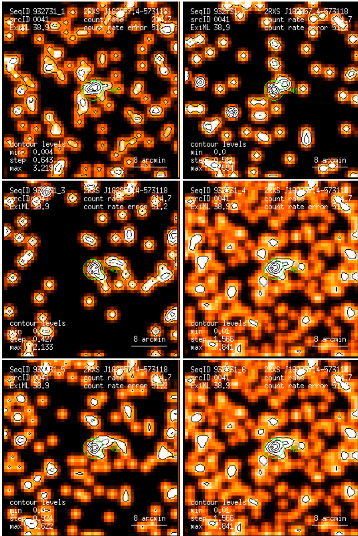
Figure 41: RASS 932731: detection 0041: band rate images, Gaussian filter: (1) PSPC channels 11 – 41, (2) 52 – 90, (3) 91 – 201, (4) 11 – 235, (5) 52 – 201, (6) 11 – 201. Broad band rates in counts/ks. Band rate contour levels in counts/ks/arcmin 2 .
