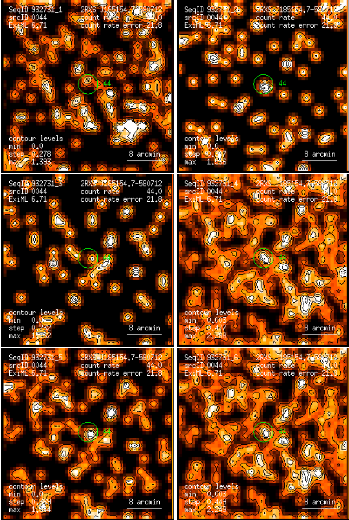
Figure 44: RASS 932731: detection 0044: band rate images, Gaussian filter: (1) PSPC channels 11 – 41, (2) 52 – 90, (3) 91 – 201, (4) 11 – 235, (5) 52 – 201, (6) 11 – 201. Broad band rates in counts/ks. Band rate contour levels in counts/ks/arcmin 2 .
