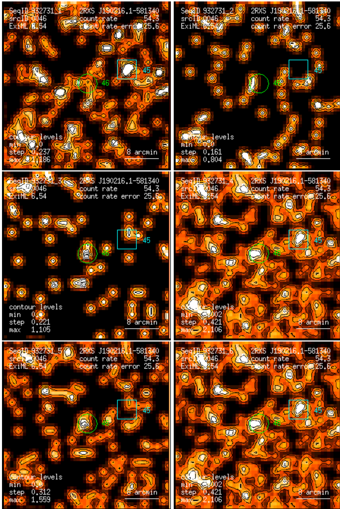
Figure 46: RASS 932731: detection 0046: band rate images, Gaussian filter: (1) PSPC channels 11 – 41, (2) 52 – 90, (3) 91 – 201, (4) 11 – 235, (5) 52 – 201, (6) 11 – 201. Broad band rates in counts/ks. Band rate contour levels in counts/ks/arcmin 2 .
