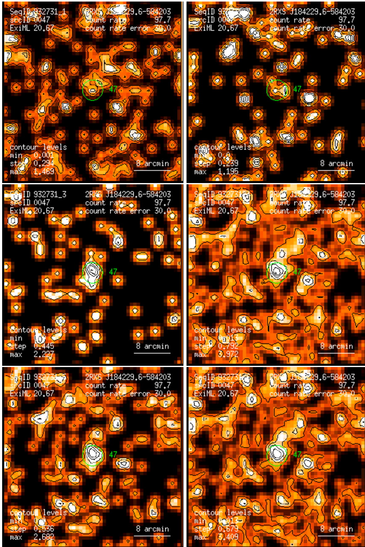
Figure 47: RASS 932731: detection 0047: band rate images, Gaussian filter: (1) PSPC channels 11 – 41, (2) 52 – 90, (3) 91 – 201, (4) 11 – 235, (5) 52 – 201, (6) 11 – 201. Broad band rates in counts/ks. Band rate contour levels in counts/ks/arcmin 2 .
