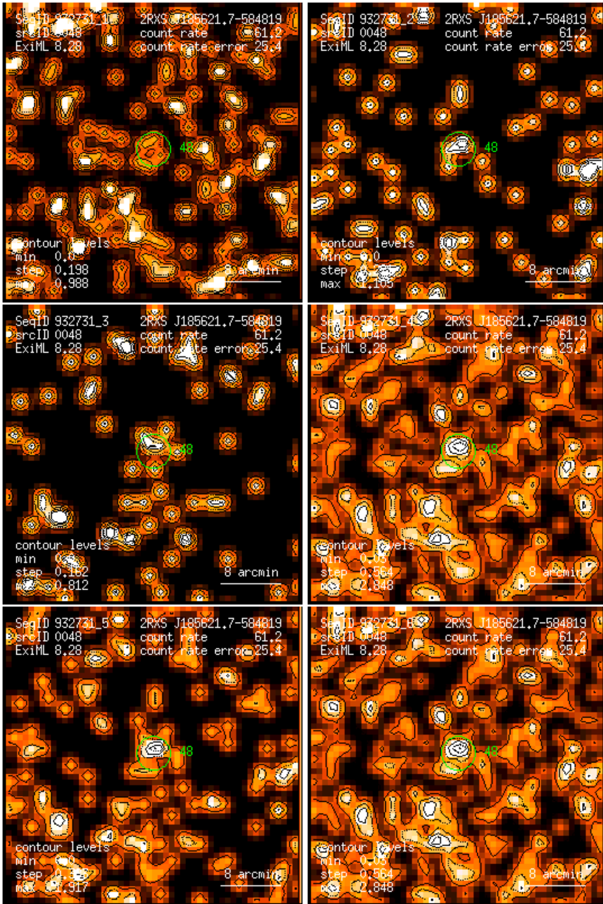
Figure 48: RASS 932731: detection 0048: band rate images, Gaussian filter: (1) PSPC channels 11 – 41, (2) 52 – 90, (3) 91 – 201, (4) 11 – 235, (5) 52 – 201, (6) 11 – 201. Broad band rates in counts/ks. Band rate contour levels in counts/ks/arcmin 2 .
