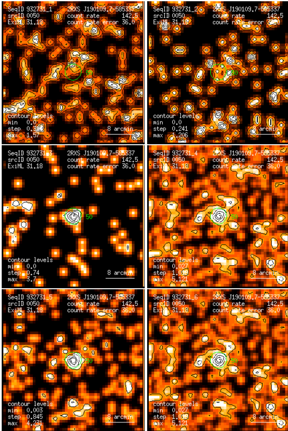
Figure 50: RASS 932731: detection 0050: band rate images, Gaussian filter: (1) PSPC channels 11 – 41, (2) 52 – 90, (3) 91 – 201, (4) 11 – 235, (5) 52 – 201, (6) 11 – 201. Broad band rates in counts/ks. Band rate contour levels in counts/ks/arcmin 2 .
