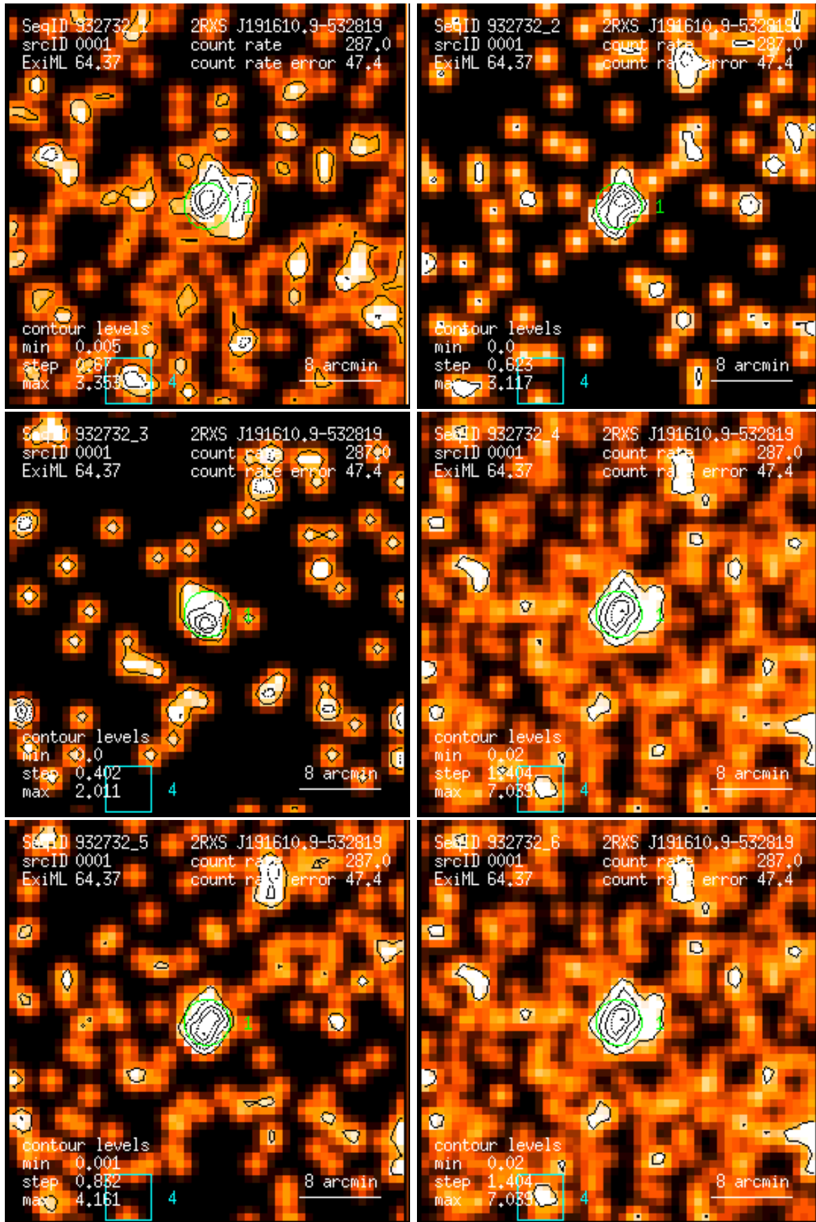
Figure 1: RASS 932732: detection 0001: band rate images, Gaussian filter: (1) PSPC channels 11 – 41, (2) 52 – 90, (3) 91 – 201, (4) 11 – 235, (5) 52 – 201, (6) 11 – 201. Broad band rates in counts/ks. Band rate contour levels in counts/ks/arcmin 2 .
