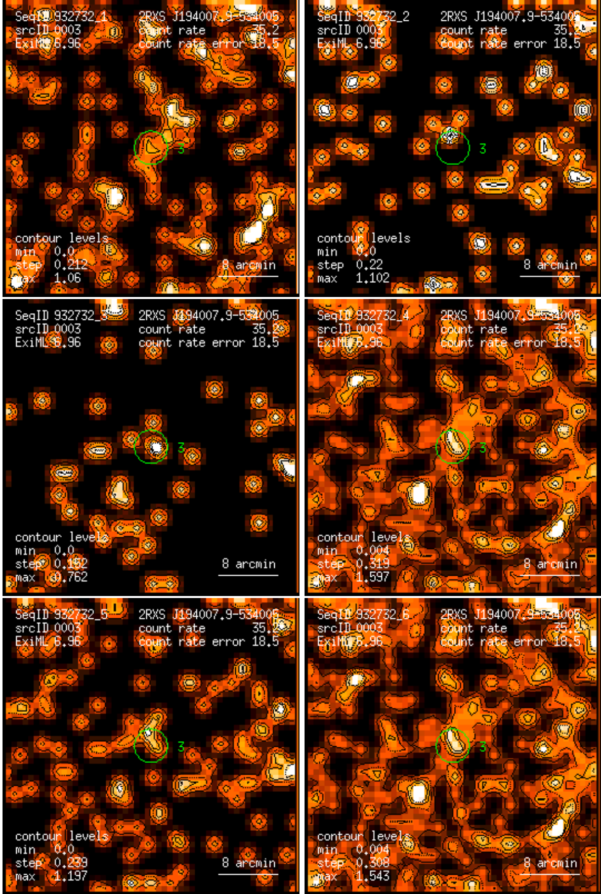
Figure 3: RASS 932732: detection 0003: band rate images, Gaussian filter: (1) PSPC channels 11 – 41, (2) 52 – 90, (3) 91 – 201, (4) 11 – 235, (5) 52 – 201, (6) 11 – 201. Broad band rates in counts/ks. Band rate contour levels in counts/ks/arcmin 2 .
