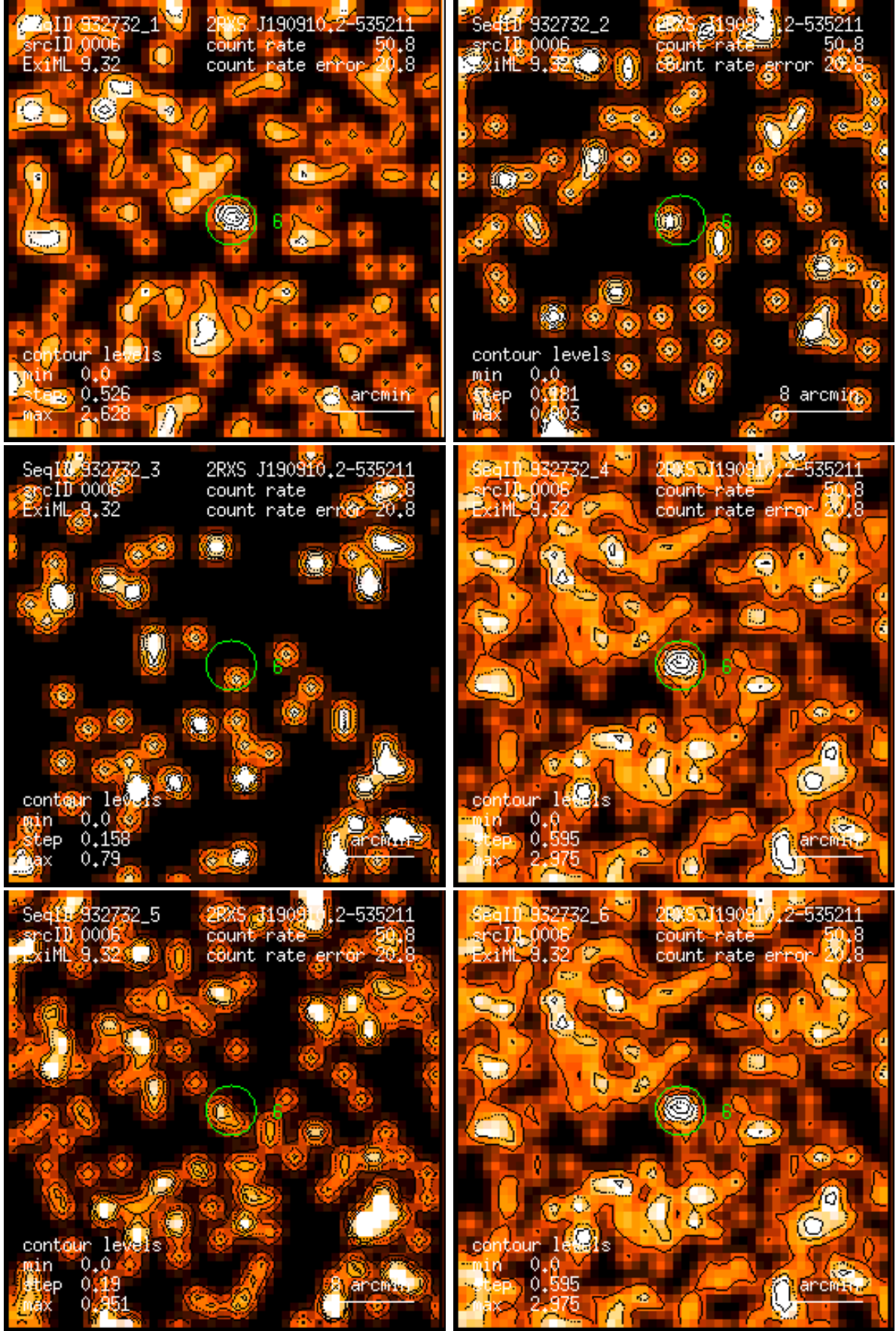
Figure 6: RASS 932732: detection 0006: band rate images, Gaussian filter: (1) PSPC channels 11 – 41, (2) 52 – 90, (3) 91 – 201, (4) 11 – 235, (5) 52 – 201, (6) 11 – 201. Broad band rates in counts/ks. Band rate contour levels in counts/ks/arcmin 2 .
