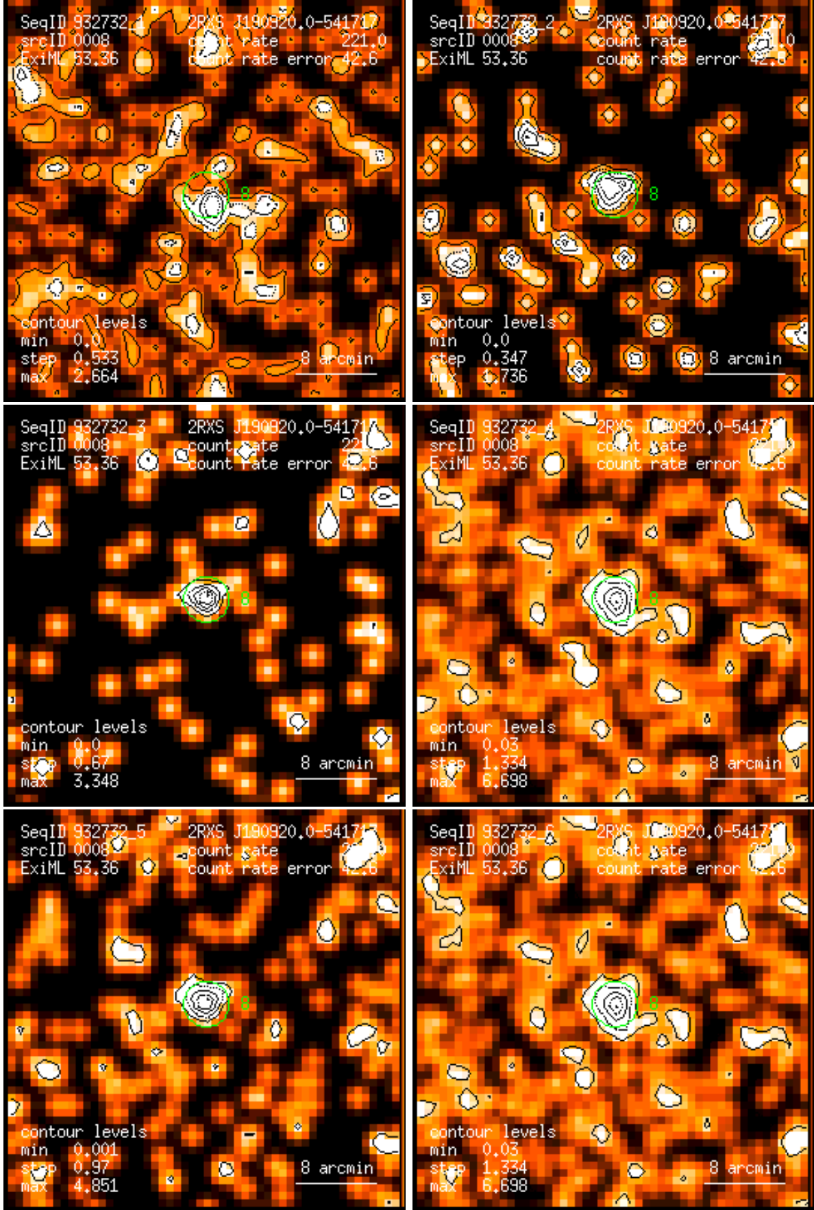
Figure 8: RASS 932732: detection 0008: band rate images, Gaussian filter: (1) PSPC channels 11 – 41, (2) 52 – 90, (3) 91 – 201, (4) 11 – 235, (5) 52 – 201, (6) 11 – 201. Broad band rates in counts/ks. Band rate contour levels in counts/ks/arcmin 2 .
