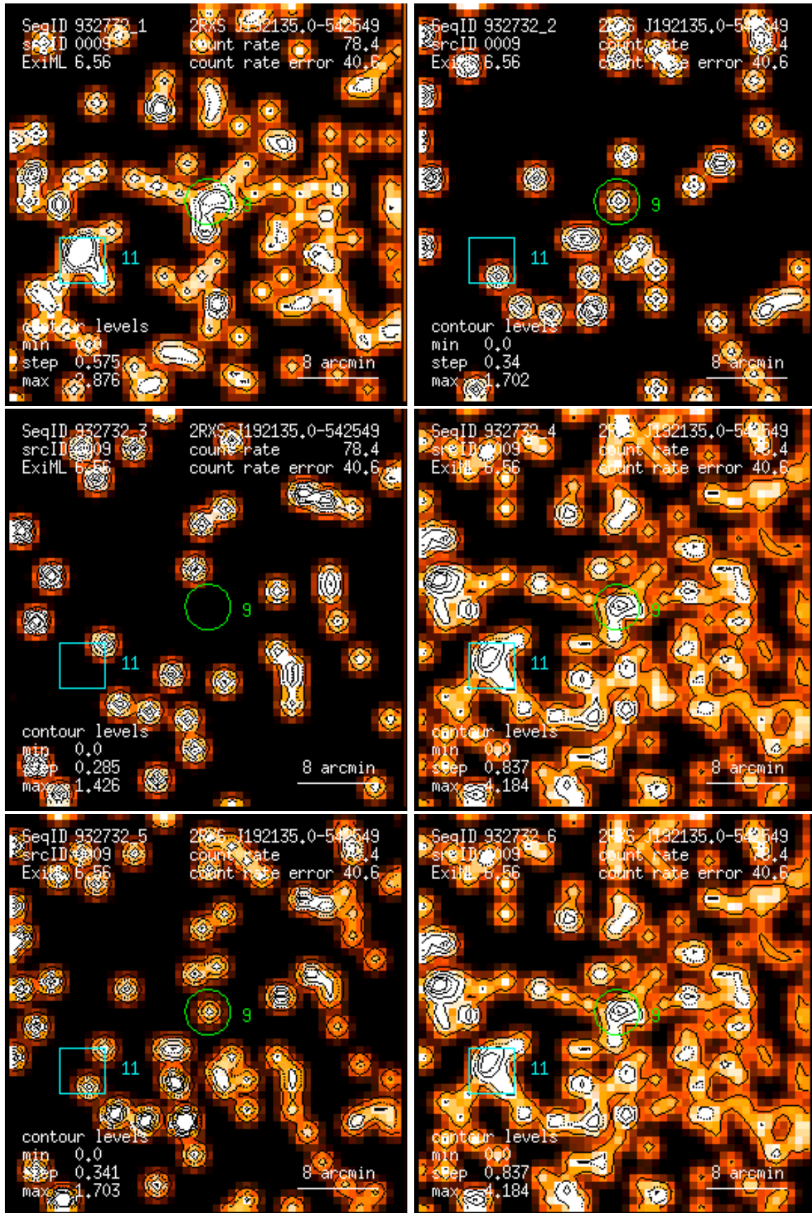
Figure 9: RASS 932732: detection 0009: band rate images, Gaussian filter: (1) PSPC channels 11 – 41, (2) 52 – 90, (3) 91 – 201, (4) 11 – 235, (5) 52 – 201, (6) 11 – 201. Broad band rates in counts/ks. Band rate contour levels in counts/ks/arcmin 2 .
