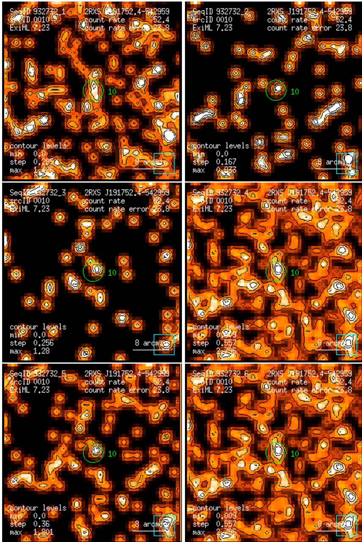
Figure 10: RASS 932732: detection 0010: band rate images, Gaussian filter: (1) PSPC channels 11 – 41, (2) 52 – 90, (3) 91 – 201, (4) 11 – 235, (5) 52 – 201, (6) 11 – 201. Broad band rates in counts/ks. Band rate contour levels in counts/ks/arcmin 2 .
