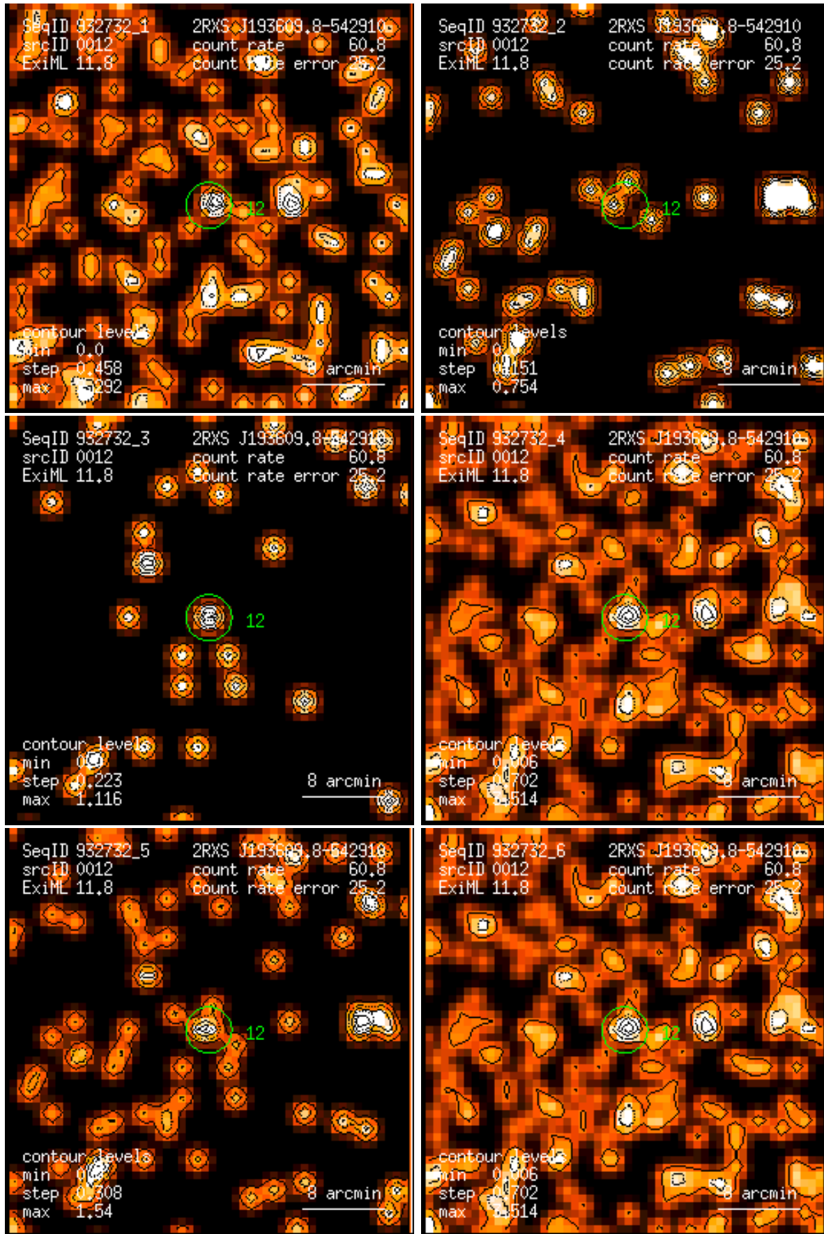
Figure 12: RASS 932732: detection 0012: band rate images, Gaussian filter: (1) PSPC channels 11 – 41, (2) 52 – 90, (3) 91 – 201, (4) 11 – 235, (5) 52 – 201, (6) 11 – 201. Broad band rates in counts/ks. Band rate contour levels in counts/ks/arcmin 2 .
