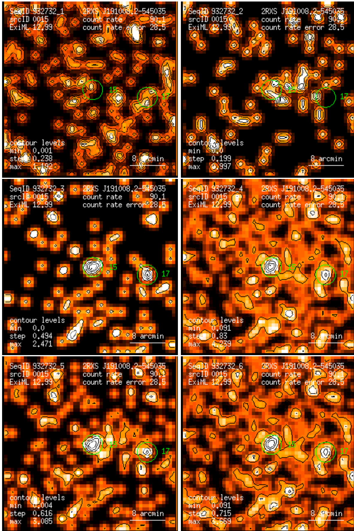
Figure 15: RASS 932732: detection 0015: band rate images, Gaussian filter: (1) PSPC channels 11 – 41, (2) 52 – 90, (3) 91 – 201, (4) 11 – 235, (5) 52 – 201, (6) 11 – 201. Broad band rates in counts/ks. Band rate contour levels in counts/ks/arcmin 2 .
