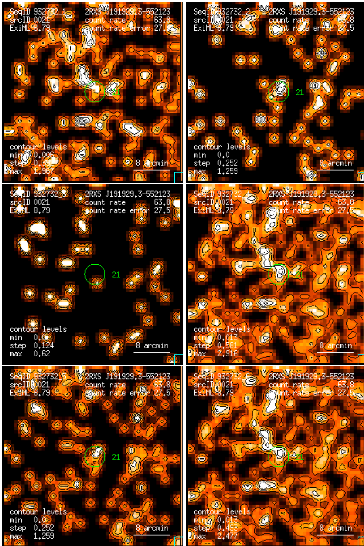
Figure 21: RASS 932732: detection 0021: band rate images, Gaussian filter: (1) PSPC channels 11 – 41, (2) 52 – 90, (3) 91 – 201, (4) 11 – 235, (5) 52 – 201, (6) 11 – 201. Broad band rates in counts/ks. Band rate contour levels in counts/ks/arcmin 2 .
