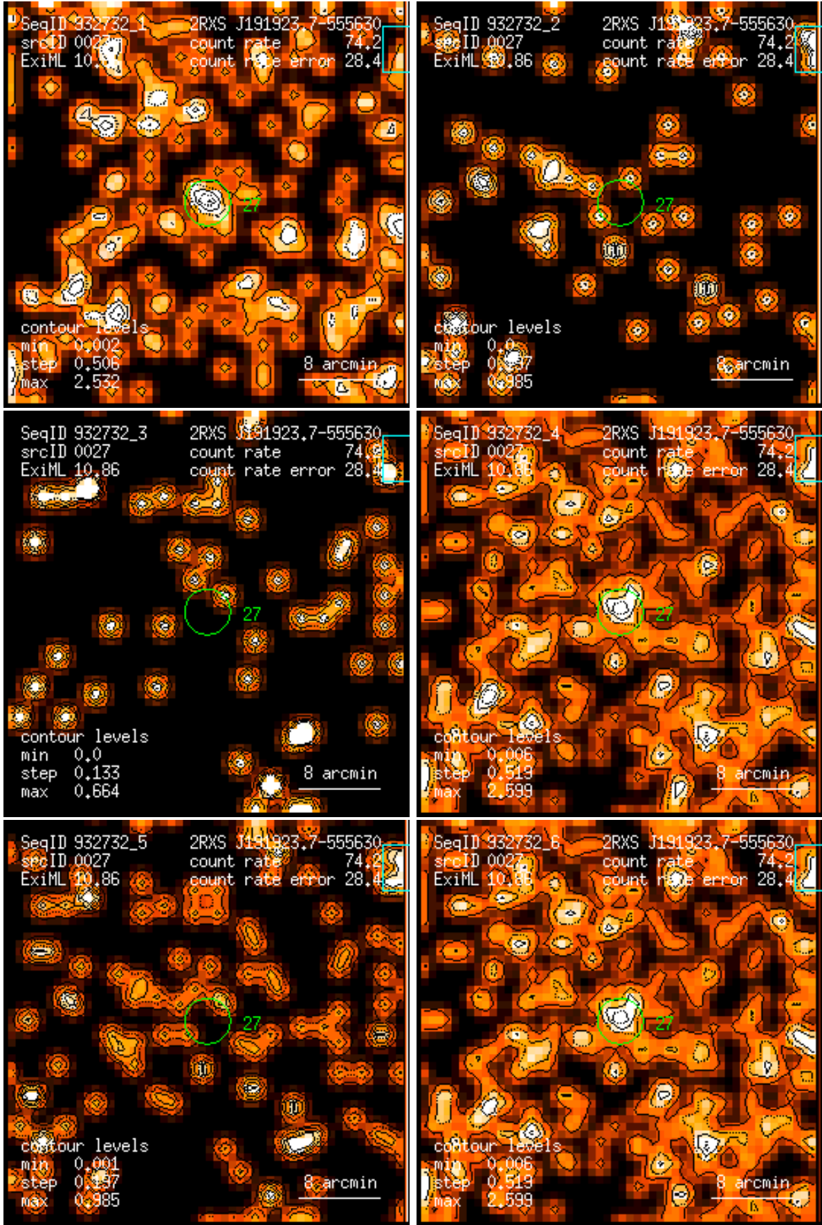
Figure 27: RASS 932732: detection 0027: band rate images, Gaussian filter: (1) PSPC channels 11 – 41, (2) 52 – 90, (3) 91 – 201, (4) 11 – 235, (5) 52 – 201, (6) 11 – 201. Broad band rates in counts/ks. Band rate contour levels in counts/ks/arcmin 2 .
