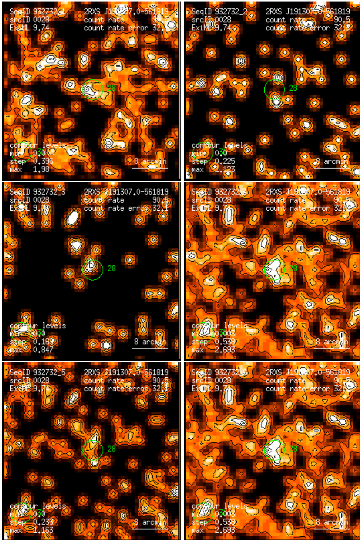
Figure 28: RASS 932732: detection 0028: band rate images, Gaussian filter: (1) PSPC channels 11 – 41, (2) 52 – 90, (3) 91 – 201, (4) 11 – 235, (5) 52 – 201, (6) 11 – 201. Broad band rates in counts/ks. Band rate contour levels in counts/ks/arcmin 2 .
