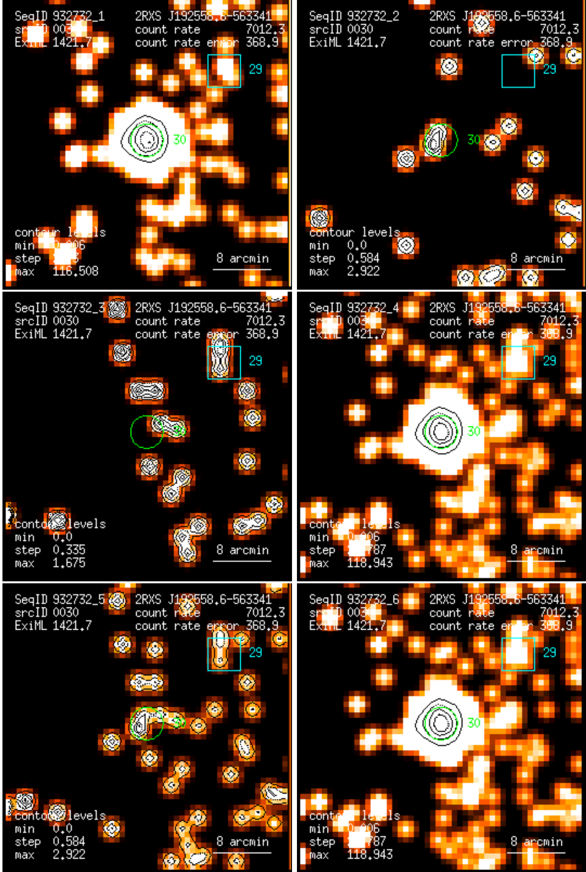
Figure 30: RASS 932732: detection 0030: band rate images, Gaussian filter: (1) PSPC channels 11 – 41, (2) 52 – 90, (3) 91 – 201, (4) 11 – 235, (5) 52 – 201, (6) 11 – 201. Broad band rates in counts/ks. Band rate contour levels in counts/ks/arcmin 2 .
