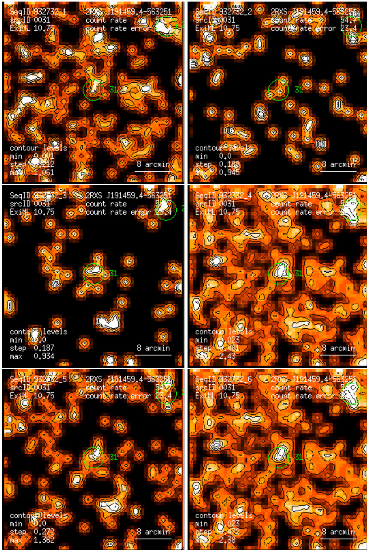
Figure 31: RASS 932732: detection 0031: band rate images, Gaussian filter: (1) PSPC channels 11 – 41, (2) 52 – 90, (3) 91 – 201, (4) 11 – 235, (5) 52 – 201, (6) 11 – 201. Broad band rates in counts/ks. Band rate contour levels in counts/ks/arcmin 2 .
