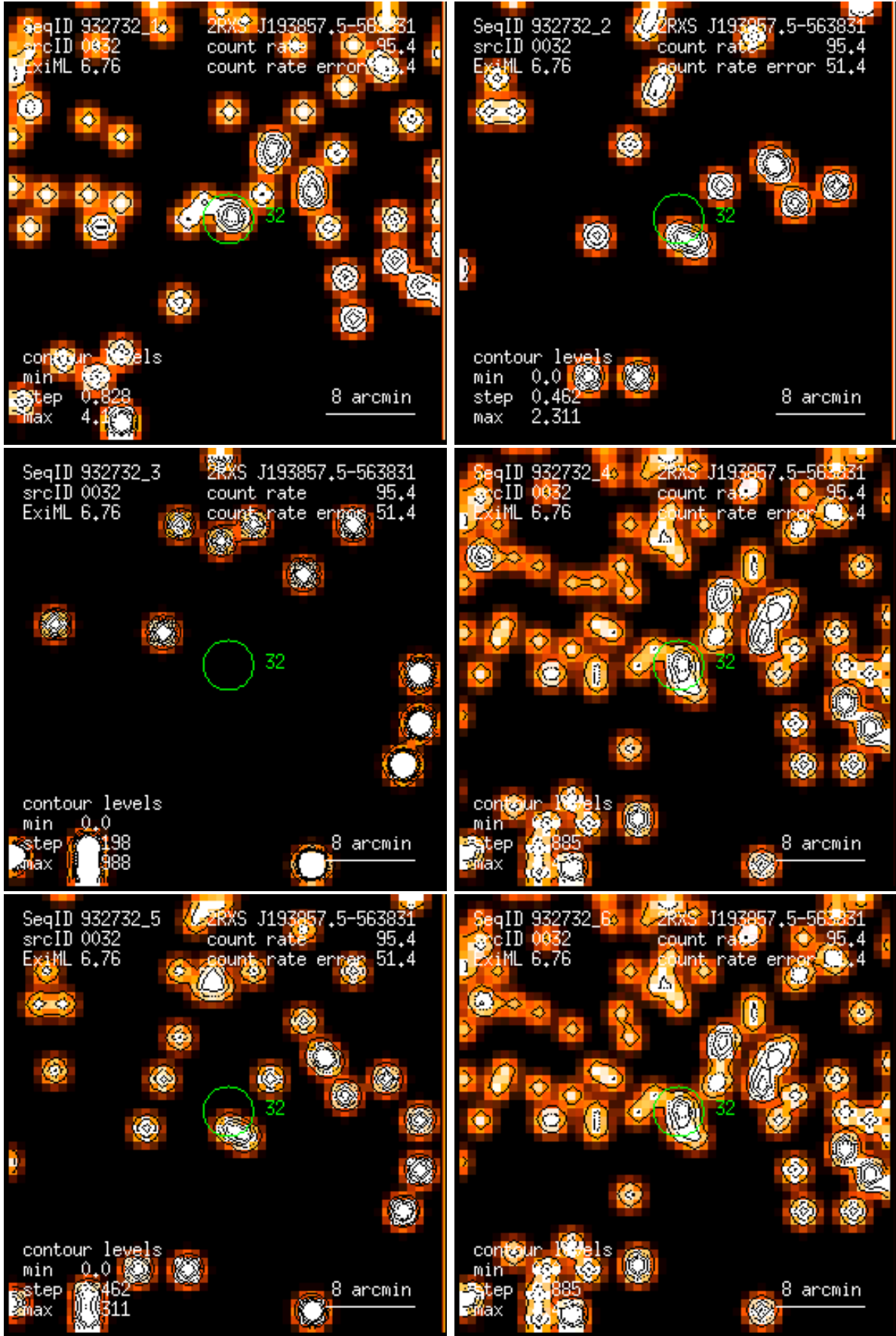
Figure 32: RASS 932732: detection 0032: band rate images, Gaussian filter: (1) PSPC channels 11 – 41, (2) 52 – 90, (3) 91 – 201, (4) 11 – 235, (5) 52 – 201, (6) 11 – 201. Broad band rates in counts/ks. Band rate contour levels in counts/ks/arcmin 2 .
