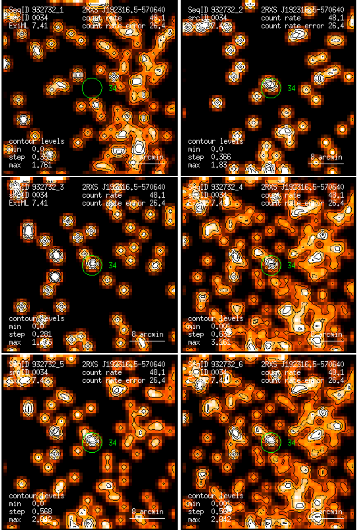
Figure 34: RASS 932732: detection 0034: band rate images, Gaussian filter: (1) PSPC channels 11 – 41, (2) 52 – 90, (3) 91 – 201, (4) 11 – 235, (5) 52 – 201, (6) 11 – 201. Broad band rates in counts/ks. Band rate contour levels in counts/ks/arcmin 2 .
