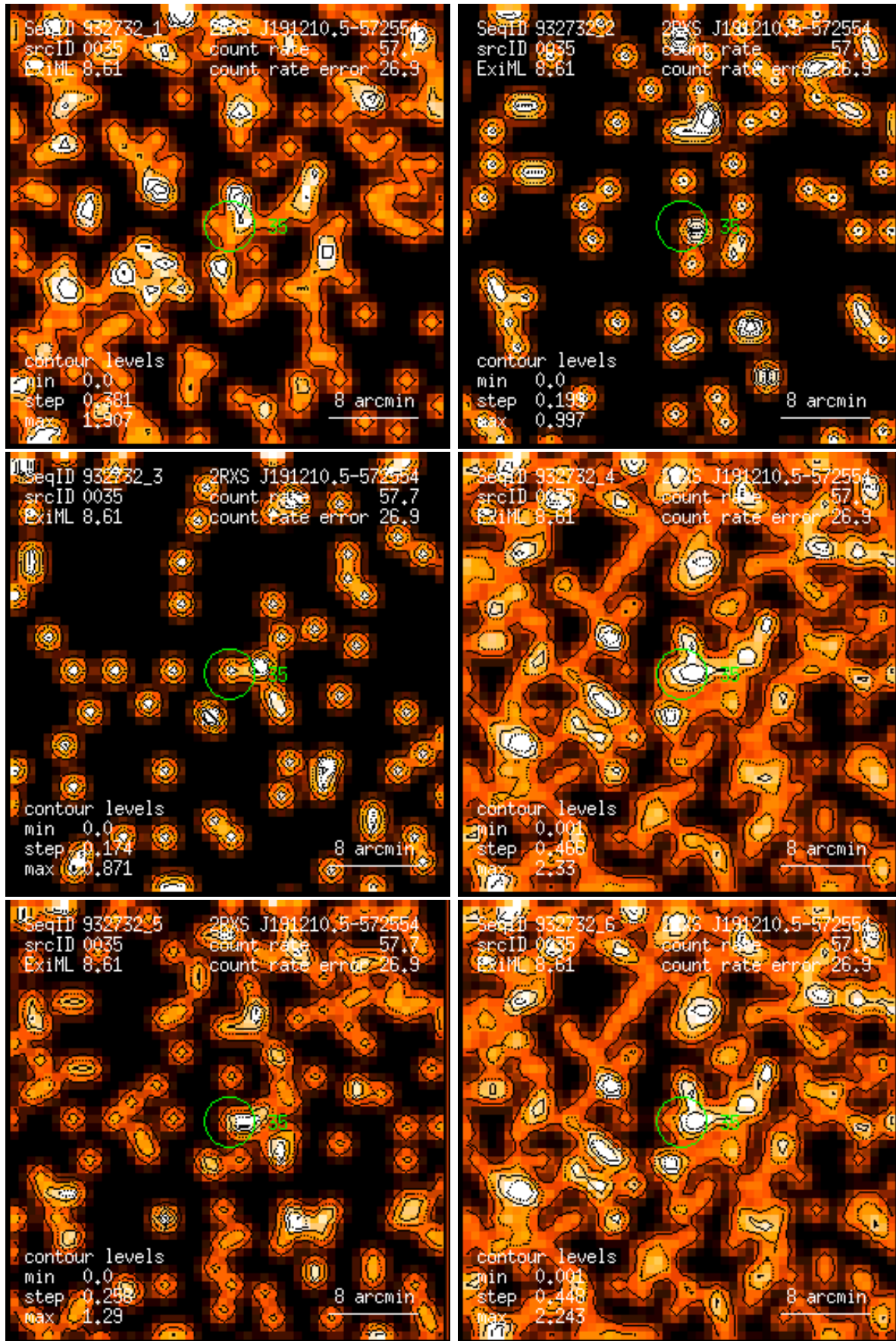
Figure 35: RASS 932732: detection 0035: band rate images, Gaussian filter: (1) PSPC channels 11 – 41, (2) 52 – 90, (3) 91 – 201, (4) 11 – 235, (5) 52 – 201, (6) 11 – 201. Broad band rates in counts/ks. Band rate contour levels in counts/ks/arcmin 2 .
