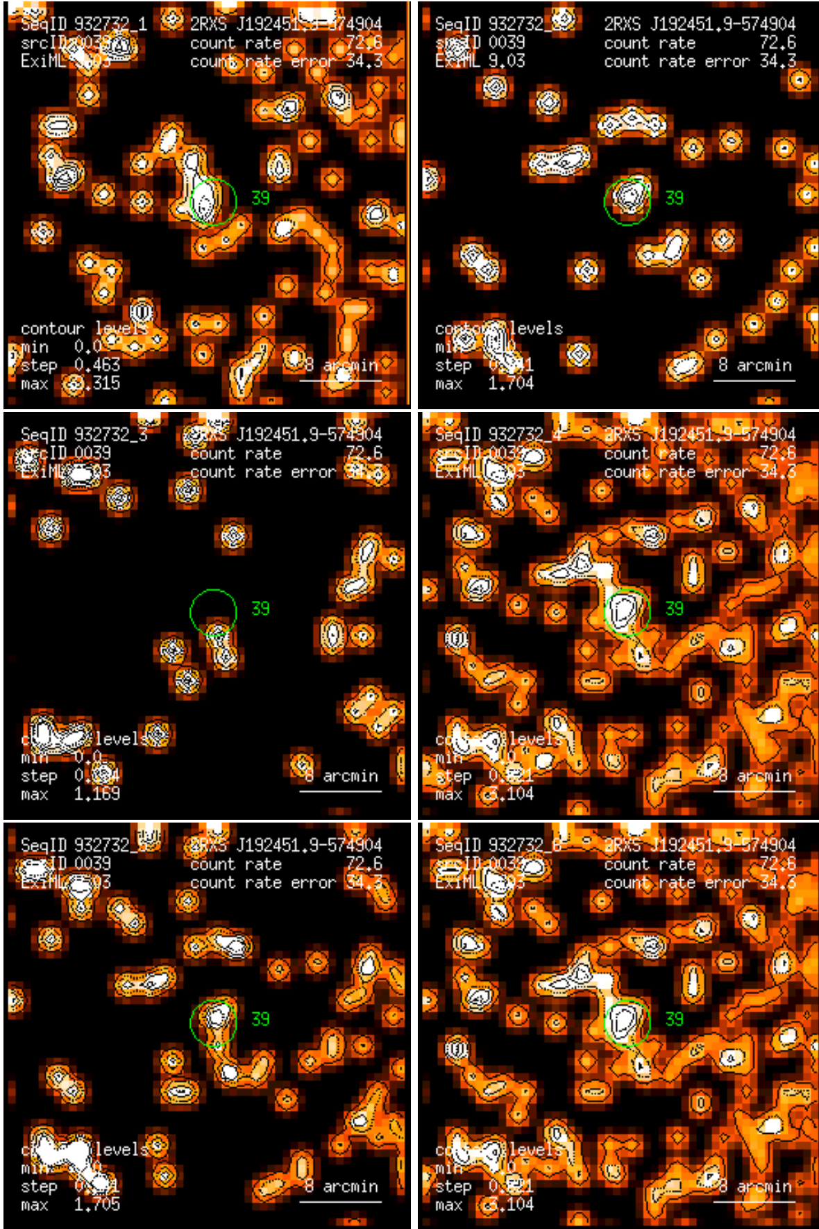
Figure 39: RASS 932732: detection 0039: band rate images, Gaussian filter: (1) PSPC channels 11 – 41, (2) 52 – 90, (3) 91 – 201, (4) 11 – 235, (5) 52 – 201, (6) 11 – 201. Broad band rates in counts/ks. Band rate contour levels in counts/ks/arcmin 2 .
