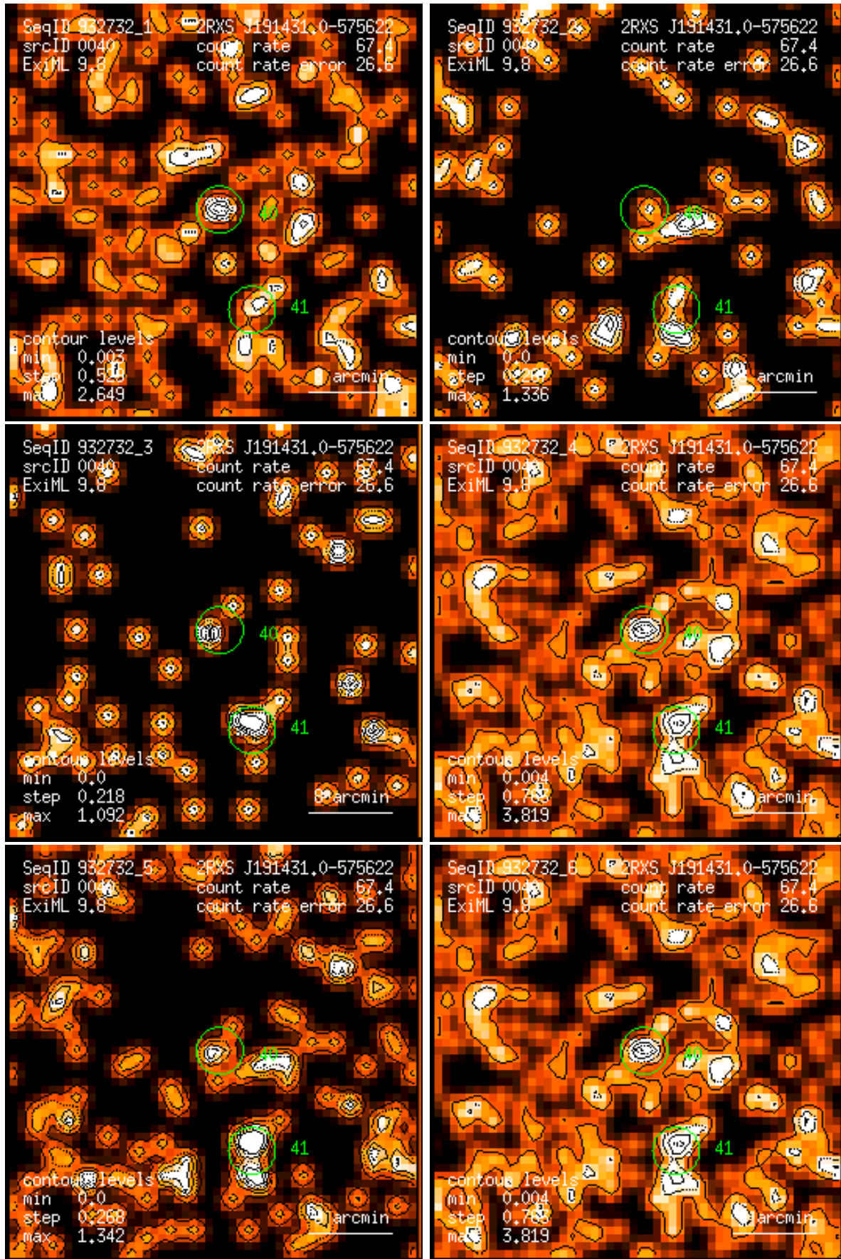
Figure 40: RASS 932732: detection 0040: band rate images, Gaussian filter: (1) PSPC channels 11 – 41, (2) 52 – 90, (3) 91 – 201, (4) 11 – 235, (5) 52 – 201, (6) 11 – 201. Broad band rates in counts/ks. Band rate contour levels in counts/ks/arcmin 2 .
