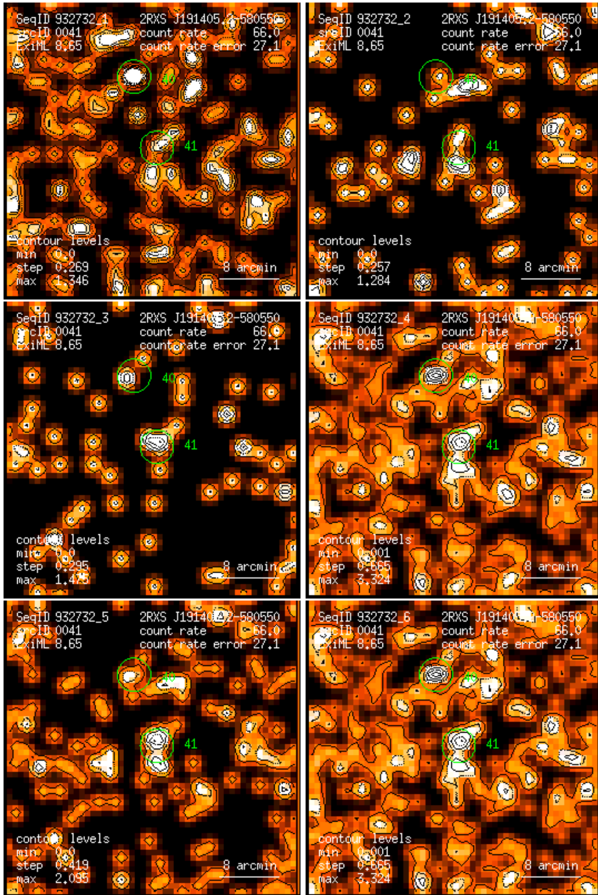
Figure 41: RASS 932732: detection 0041: band rate images, Gaussian filter: (1) PSPC channels 11 – 41, (2) 52 – 90, (3) 91 – 201, (4) 11 – 235, (5) 52 – 201, (6) 11 – 201. Broad band rates in counts/ks. Band rate contour levels in counts/ks/arcmin 2 .
