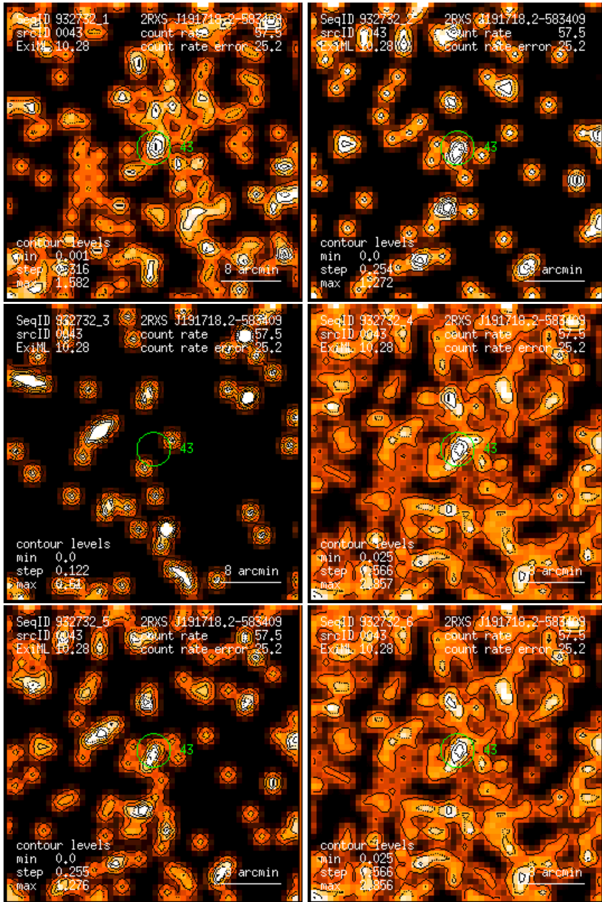
Figure 43: RASS 932732: detection 0043: band rate images, Gaussian filter: (1) PSPC channels 11 – 41, (2) 52 – 90, (3) 91 – 201, (4) 11 – 235, (5) 52 – 201, (6) 11 – 201. Broad band rates in counts/ks. Band rate contour levels in counts/ks/arcmin 2 .
