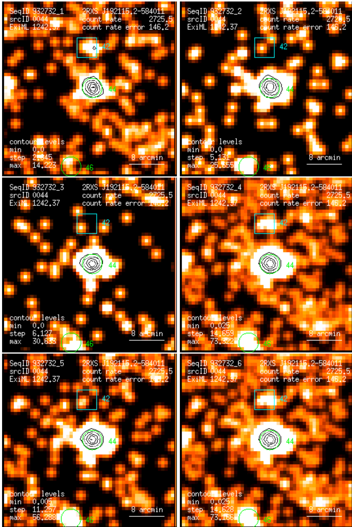
Figure 44: RASS 932732: detection 0044: band rate images, Gaussian filter: (1) PSPC channels 11 – 41, (2) 52 – 90, (3) 91 – 201, (4) 11 – 235, (5) 52 – 201, (6) 11 – 201. Broad band rates in counts/ks. Band rate contour levels in counts/ks/arcmin 2 .
