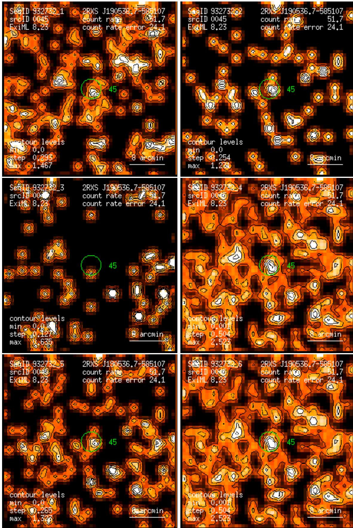
Figure 45: RASS 932732: detection 0045: band rate images, Gaussian filter: (1) PSPC channels 11 – 41, (2) 52 – 90, (3) 91 – 201, (4) 11 – 235, (5) 52 – 201, (6) 11 – 201. Broad band rates in counts/ks. Band rate contour levels in counts/ks/arcmin 2 .
