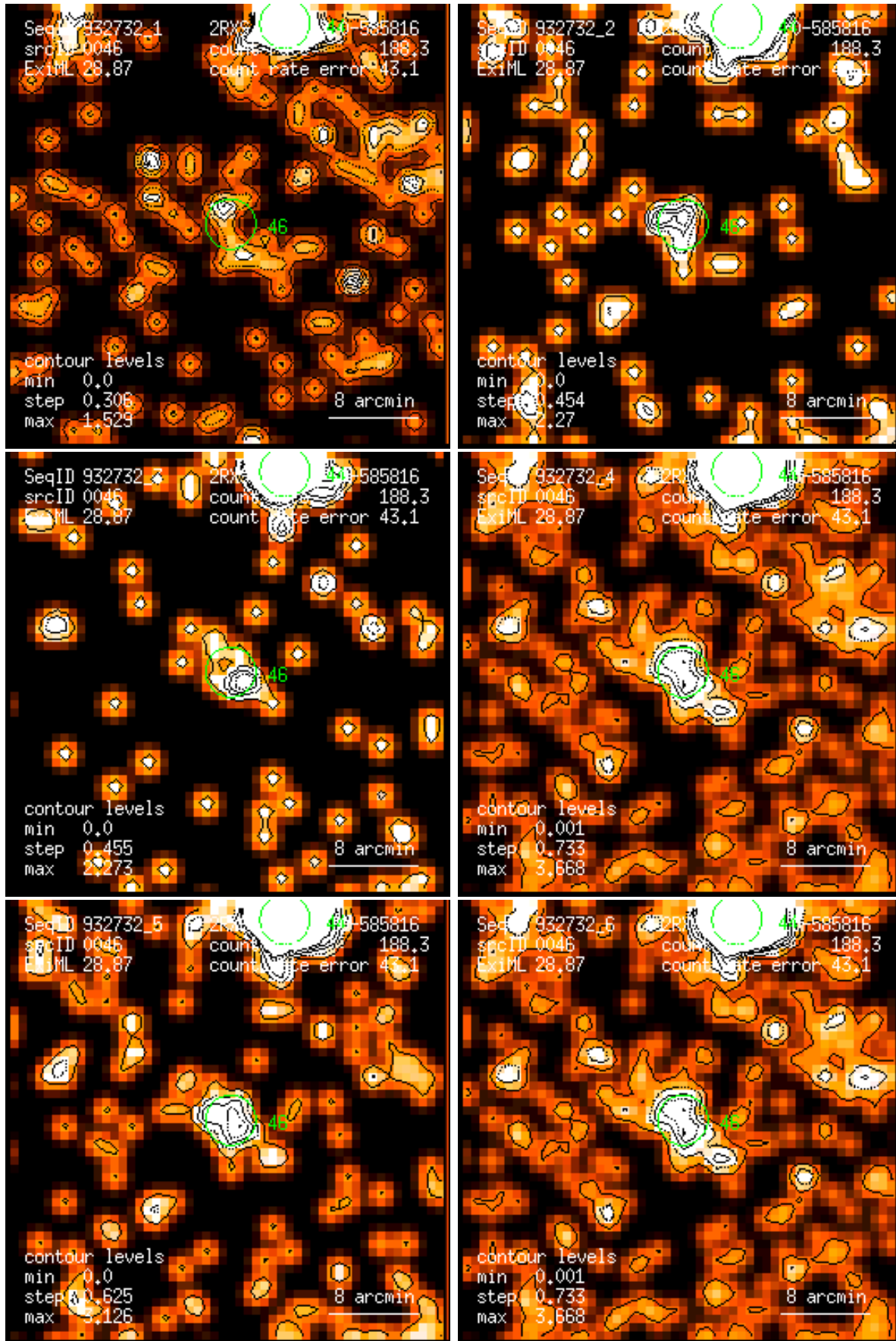
Figure 46: RASS 932732: detection 0046: band rate images, Gaussian filter: (1) PSPC channels 11 – 41, (2) 52 – 90, (3) 91 – 201, (4) 11 – 235, (5) 52 – 201, (6) 11 – 201. Broad band rates in counts/ks. Band rate contour levels in counts/ks/arcmin 2 .
