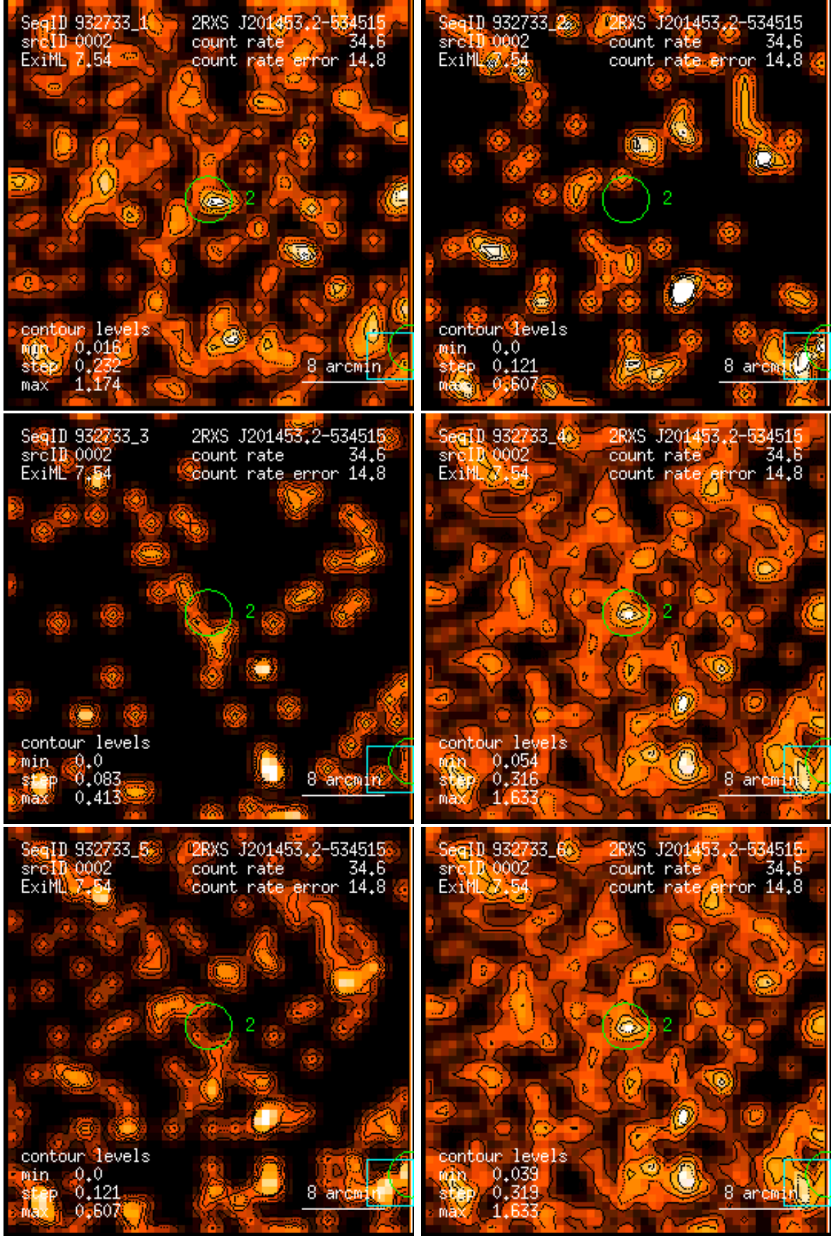
Figure 2: RASS 932733: detection 0002: band rate images, Gaussian filter: (1) PSPC channels 11 – 41, (2) 52 – 90, (3) 91 – 201, (4) 11 – 235, (5) 52 – 201, (6) 11 – 201. Broad band rates in counts/ks. Band rate contour levels in counts/ks/arcmin 2 .
