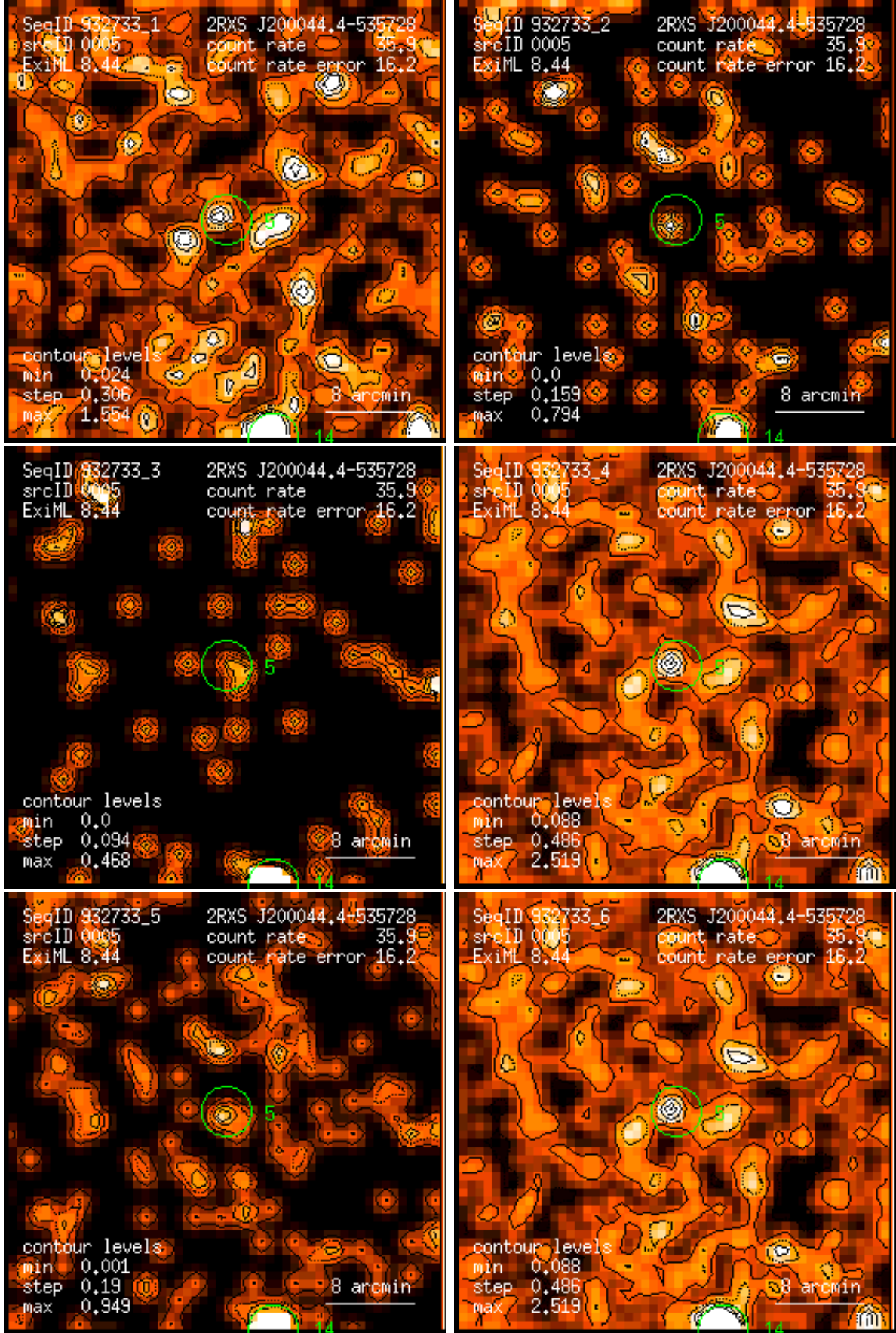
Figure 5: RASS 932733: detection 0005: band rate images, Gaussian filter: (1) PSPC channels 11 – 41, (2) 52 – 90, (3) 91 – 201, (4) 11 – 235, (5) 52 – 201, (6) 11 – 201. Broad band rates in counts/ks. Band rate contour levels in counts/ks/arcmin 2 .
