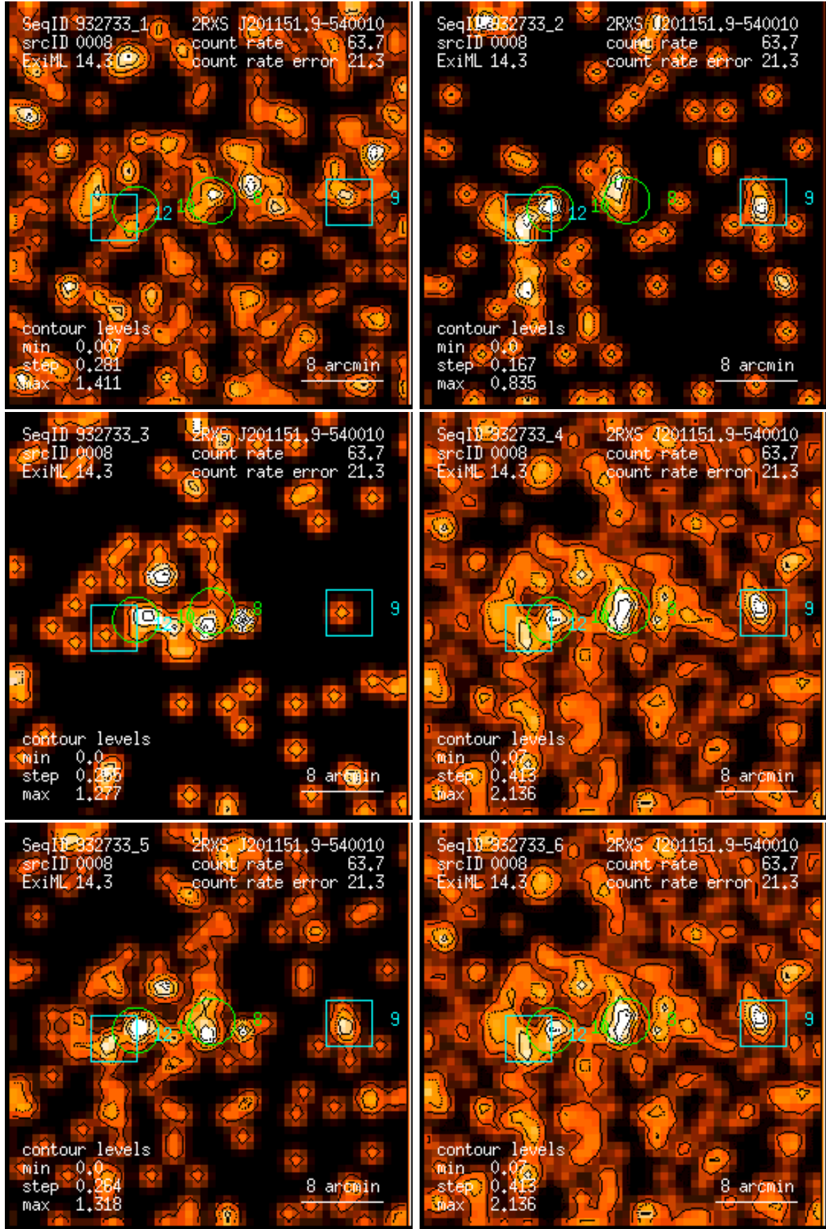
Figure 8: RASS 932733: detection 0008: band rate images, Gaussian filter: (1) PSPC channels 11 – 41, (2) 52 – 90, (3) 91 – 201, (4) 11 – 235, (5) 52 – 201, (6) 11 – 201. Broad band rates in counts/ks. Band rate contour levels in counts/ks/arcmin 2 .
