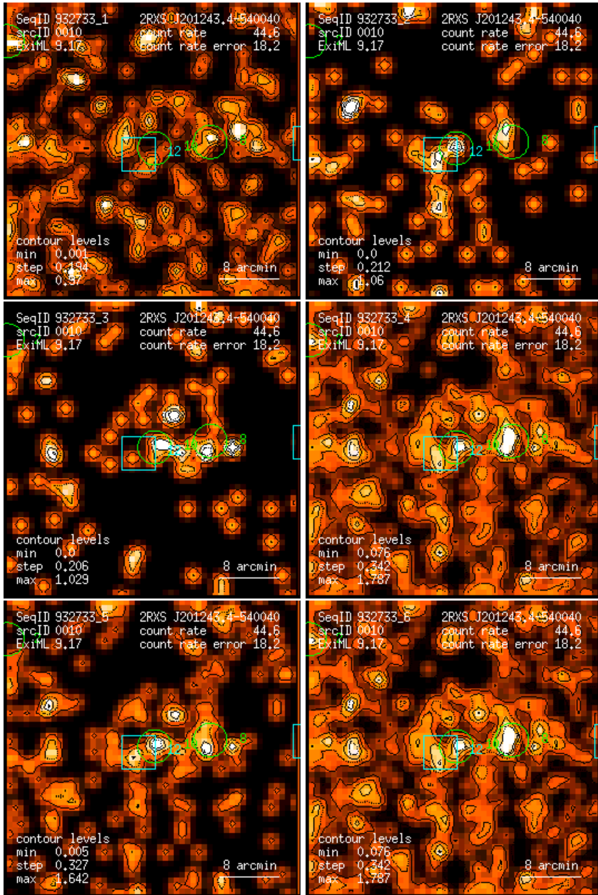
Figure 10: RASS 932733: detection 0010: band rate images, Gaussian filter: (1) PSPC channels 11 – 41, (2) 52 – 90, (3) 91 – 201, (4) 11 – 235, (5) 52 – 201, (6) 11 – 201. Broad band rates in counts/ks. Band rate contour levels in counts/ks/arcmin 2 .
