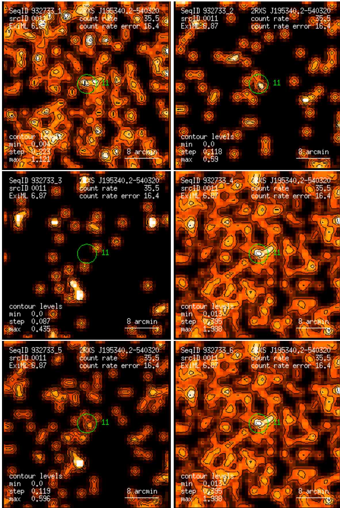
Figure 11: RASS 932733: detection 0011: band rate images, Gaussian filter: (1) PSPC channels 11 – 41, (2) 52 – 90, (3) 91 – 201, (4) 11 – 235, (5) 52 – 201, (6) 11 – 201. Broad band rates in counts/ks. Band rate contour levels in counts/ks/arcmin 2 .
