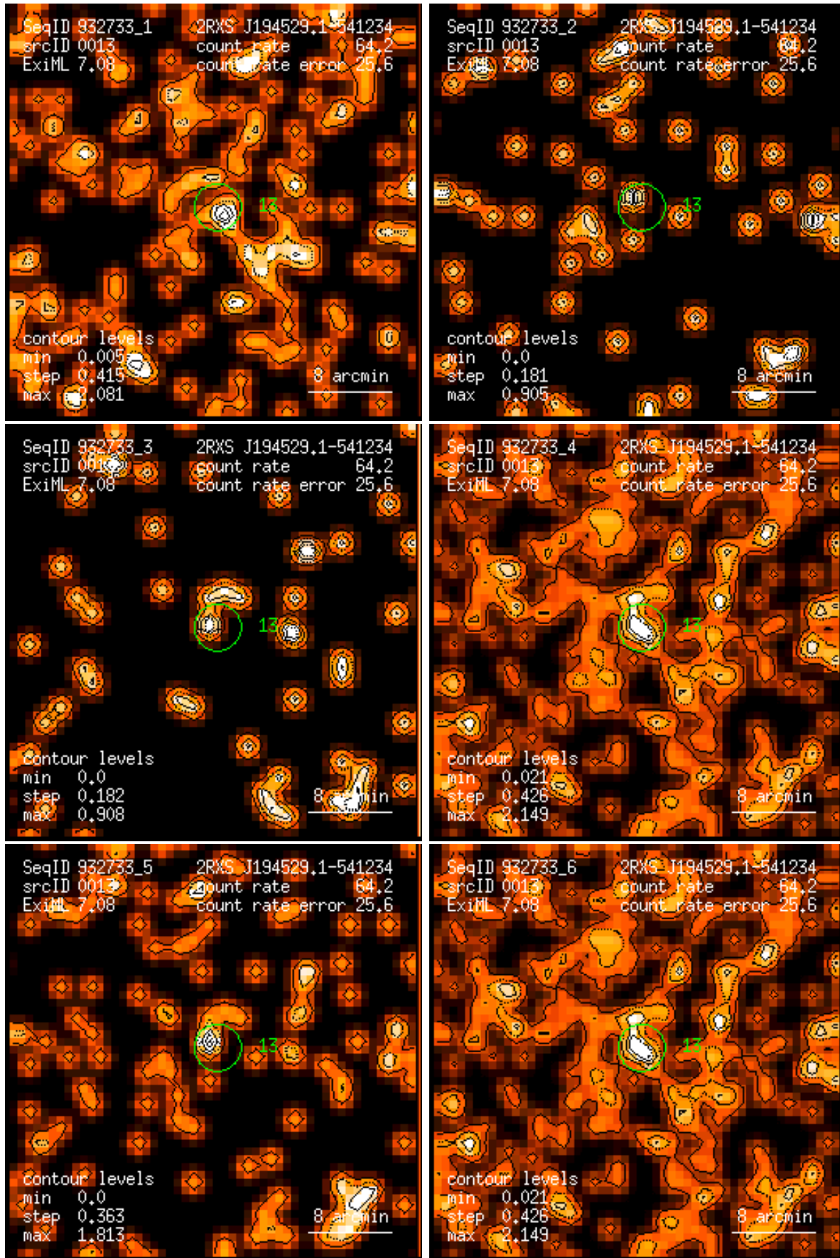
Figure 13: RASS 932733: detection 0013: band rate images, Gaussian filter: (1) PSPC channels 11 – 41, (2) 52 – 90, (3) 91 – 201, (4) 11 – 235, (5) 52 – 201, (6) 11 – 201. Broad band rates in counts/ks. Band rate contour levels in counts/ks/arcmin 2 .
