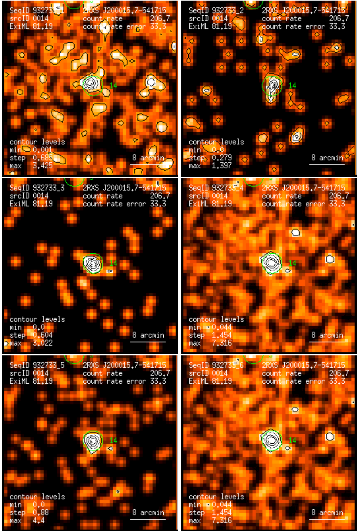
Figure 14: RASS 932733: detection 0014: band rate images, Gaussian filter: (1) PSPC channels 11 – 41, (2) 52 – 90, (3) 91 – 201, (4) 11 – 235, (5) 52 – 201, (6) 11 – 201. Broad band rates in counts/ks. Band rate contour levels in counts/ks/arcmin 2 .
