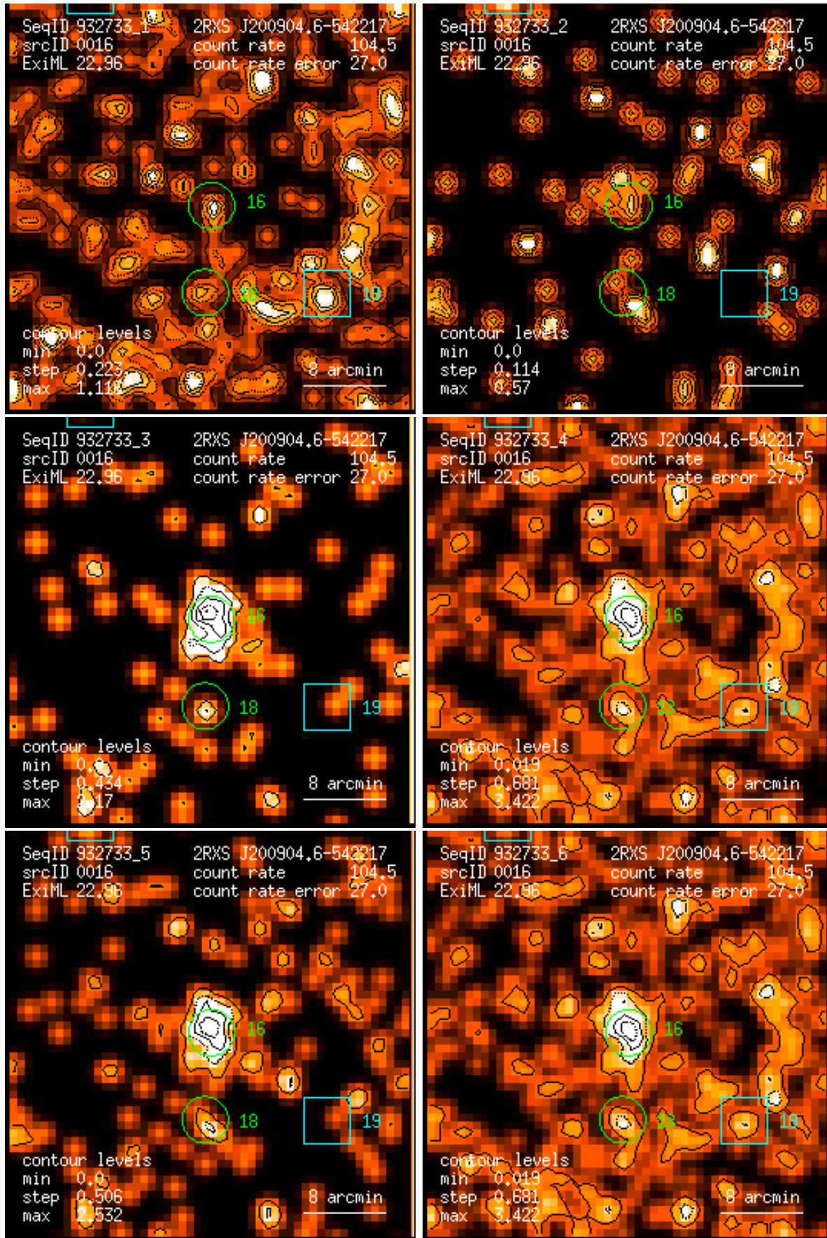
Figure 16: RASS 932733: detection 0016: band rate images, Gaussian filter: (1) PSPC channels 11 – 41, (2) 52 – 90, (3) 91 – 201, (4) 11 – 235, (5) 52 – 201, (6) 11 – 201. Broad band rates in counts/ks. Band rate contour levels in counts/ks/arcmin 2 .
