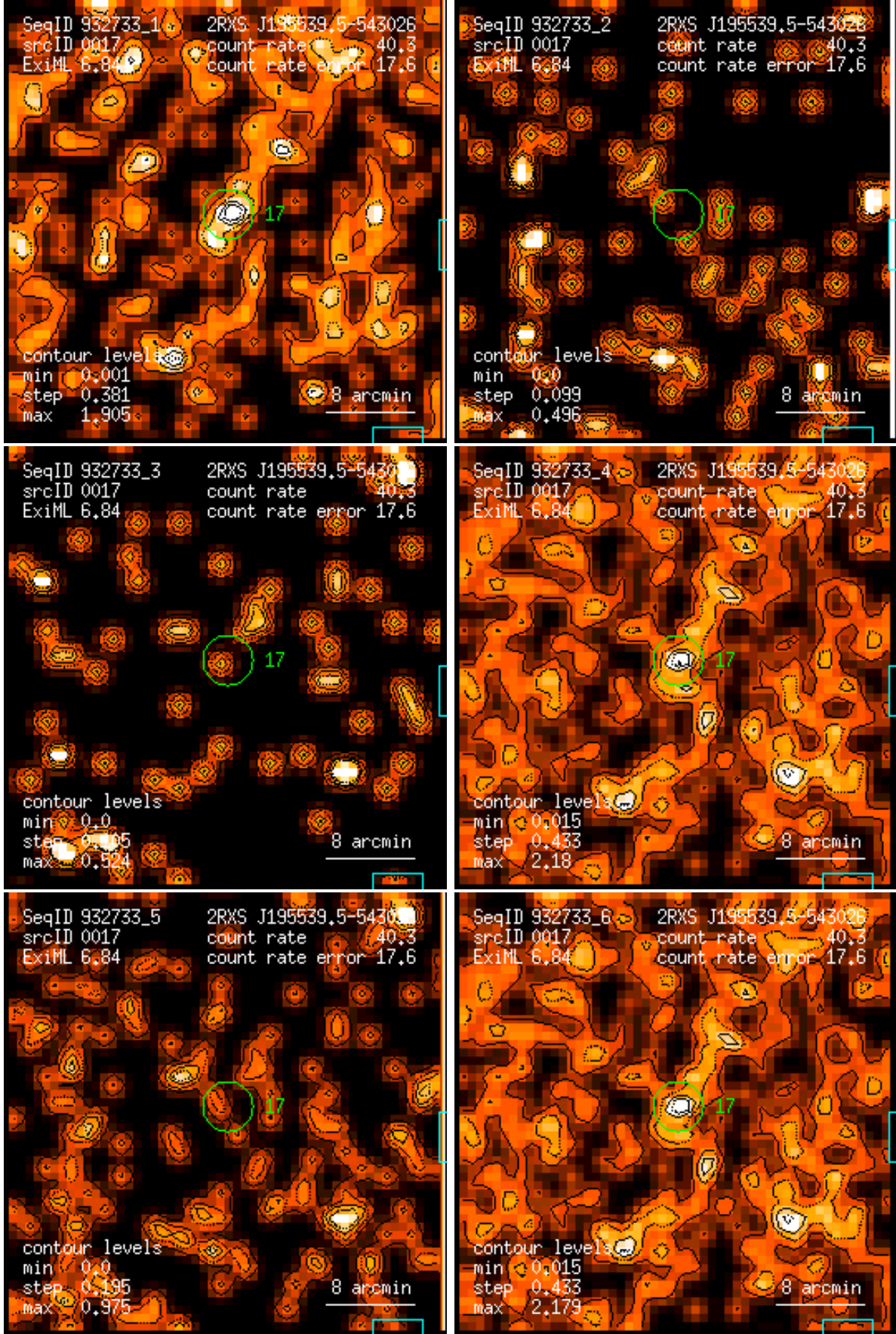
Figure 17: RASS 932733: detection 0017: band rate images, Gaussian filter: (1) PSPC channels 11 – 41, (2) 52 – 90, (3) 91 – 201, (4) 11 – 235, (5) 52 – 201, (6) 11 – 201. Broad band rates in counts/ks. Band rate contour levels in counts/ks/arcmin 2 .
