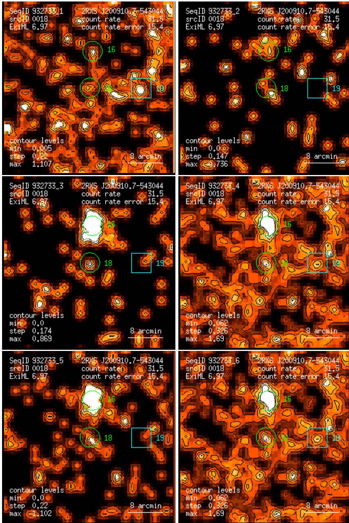
Figure 18: RASS 932733: detection 0018: band rate images, Gaussian filter: (1) PSPC channels 11 – 41, (2) 52 – 90, (3) 91 – 201, (4) 11 – 235, (5) 52 – 201, (6) 11 – 201. Broad band rates in counts/ks. Band rate contour levels in counts/ks/arcmin 2 .
