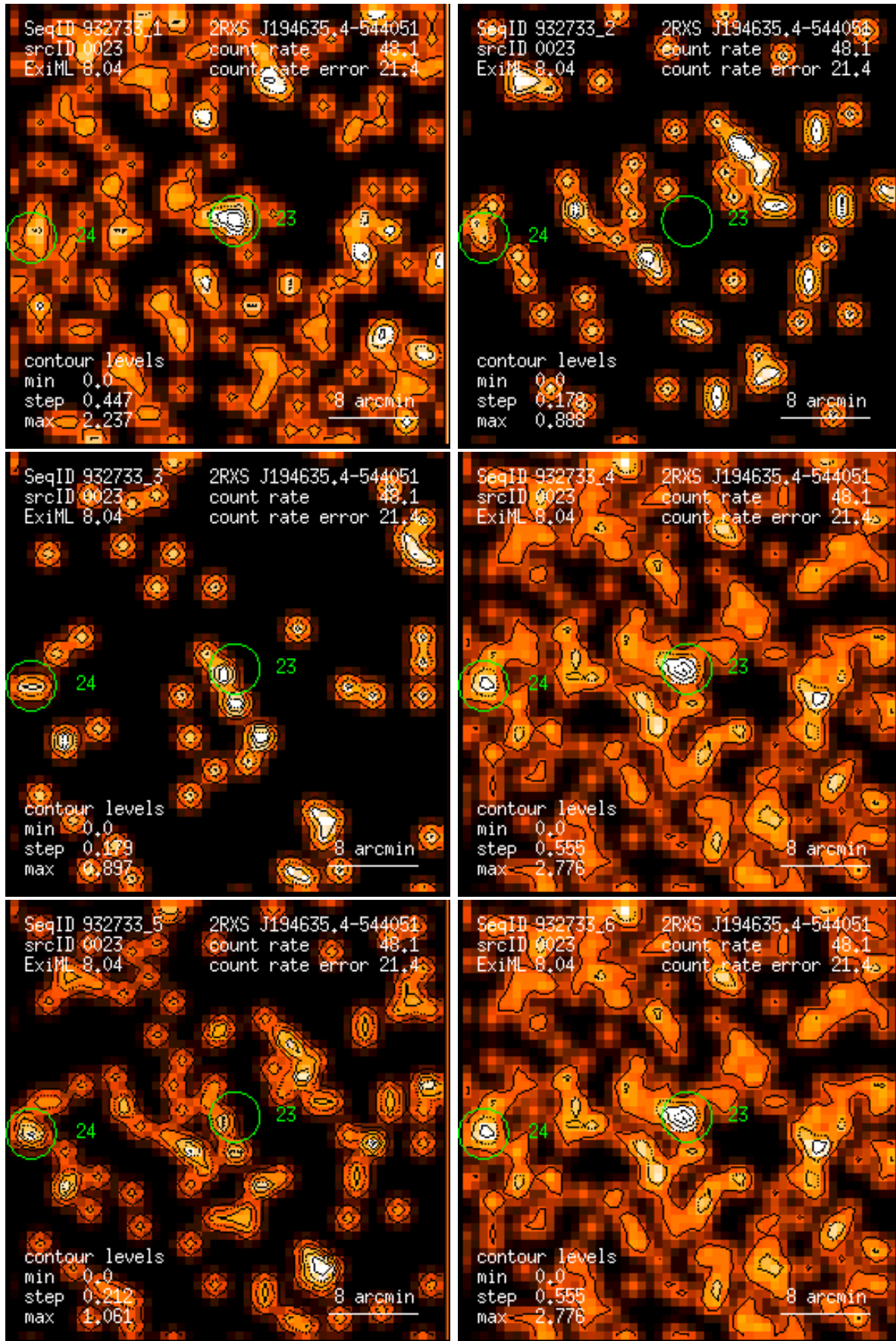
Figure 23: RASS 932733: detection 0023: band rate images, Gaussian filter: (1) PSPC channels 11 – 41, (2) 52 – 90, (3) 91 – 201, (4) 11 – 235, (5) 52 – 201, (6) 11 – 201. Broad band rates in counts/ks. Band rate contour levels in counts/ks/arcmin 2 .
