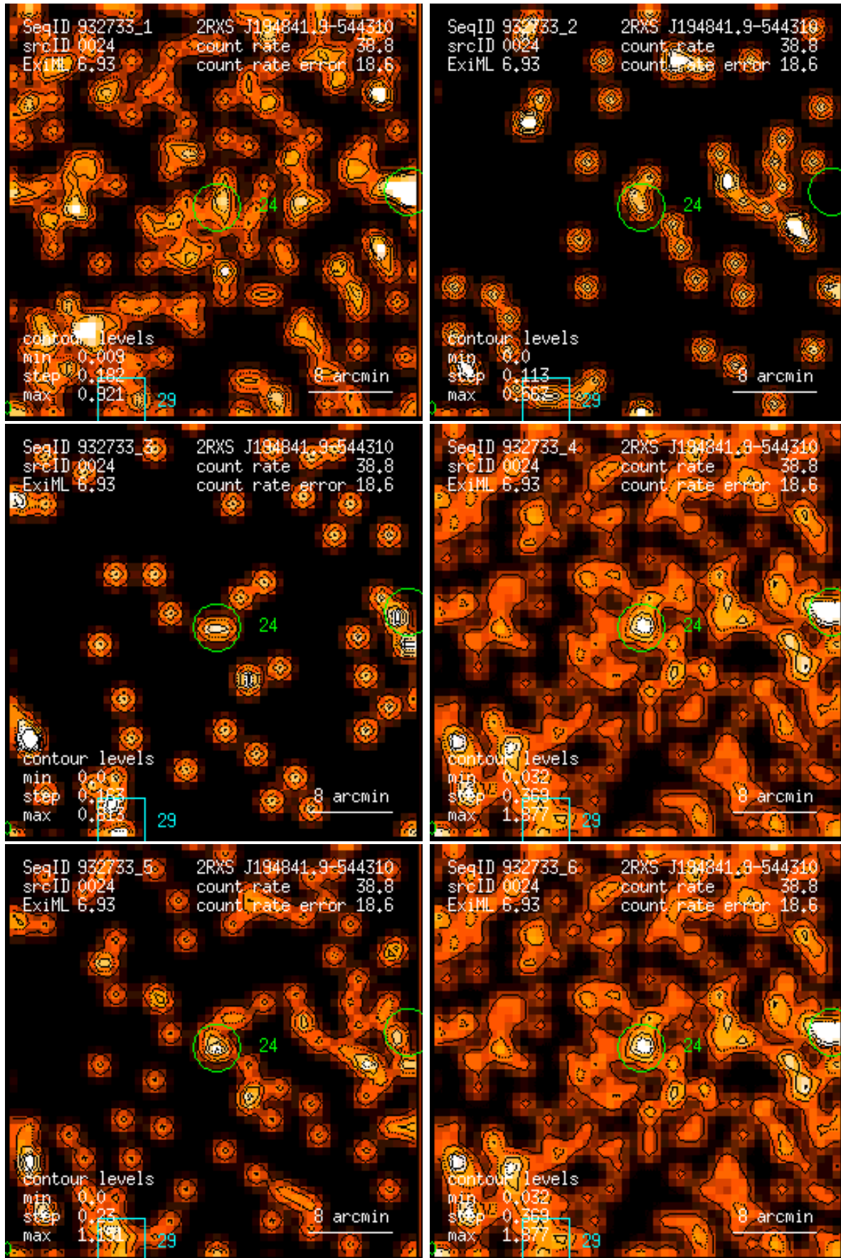
Figure 24: RASS 932733: detection 0024: band rate images, Gaussian filter: (1) PSPC channels 11 – 41, (2) 52 – 90, (3) 91 – 201, (4) 11 – 235, (5) 52 – 201, (6) 11 – 201. Broad band rates in counts/ks. Band rate contour levels in counts/ks/arcmin 2 .
