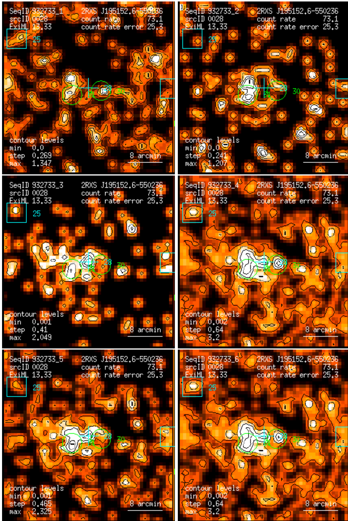
Figure 28: RASS 932733: detection 0028: band rate images, Gaussian filter: (1) PSPC channels 11 – 41, (2) 52 – 90, (3) 91 – 201, (4) 11 – 235, (5) 52 – 201, (6) 11 – 201. Broad band rates in counts/ks. Band rate contour levels in counts/ks/arcmin 2 .
