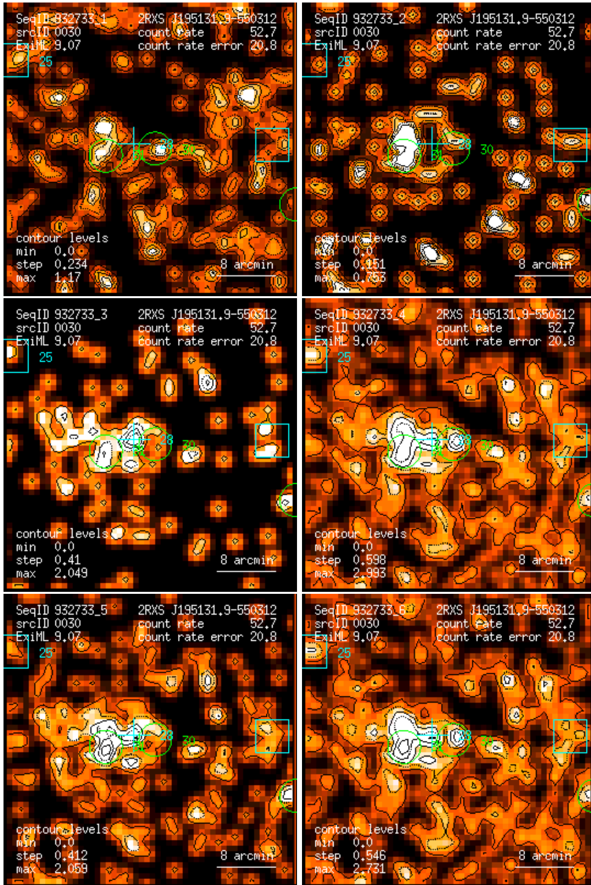
Figure 30: RASS 932733: detection 0030: band rate images, Gaussian filter: (1) PSPC channels 11 – 41, (2) 52 – 90, (3) 91 – 201, (4) 11 – 235, (5) 52 – 201, (6) 11 – 201. Broad band rates in counts/ks. Band rate contour levels in counts/ks/arcmin 2 .
