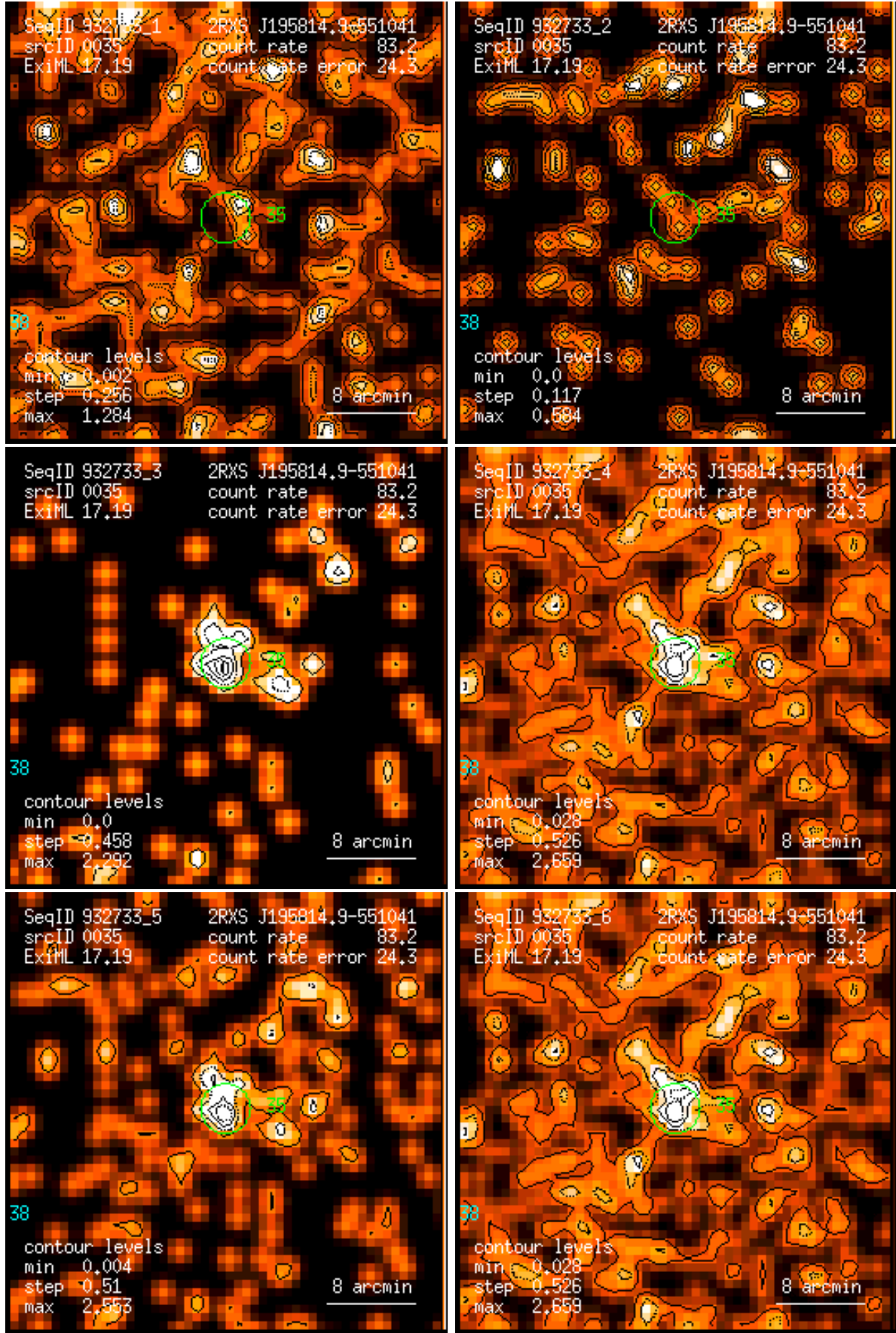
Figure 35: RASS 932733: detection 0035: band rate images, Gaussian filter: (1) PSPC channels 11 – 41, (2) 52 – 90, (3) 91 – 201, (4) 11 – 235, (5) 52 – 201, (6) 11 – 201. Broad band rates in counts/ks. Band rate contour levels in counts/ks/arcmin 2 .
