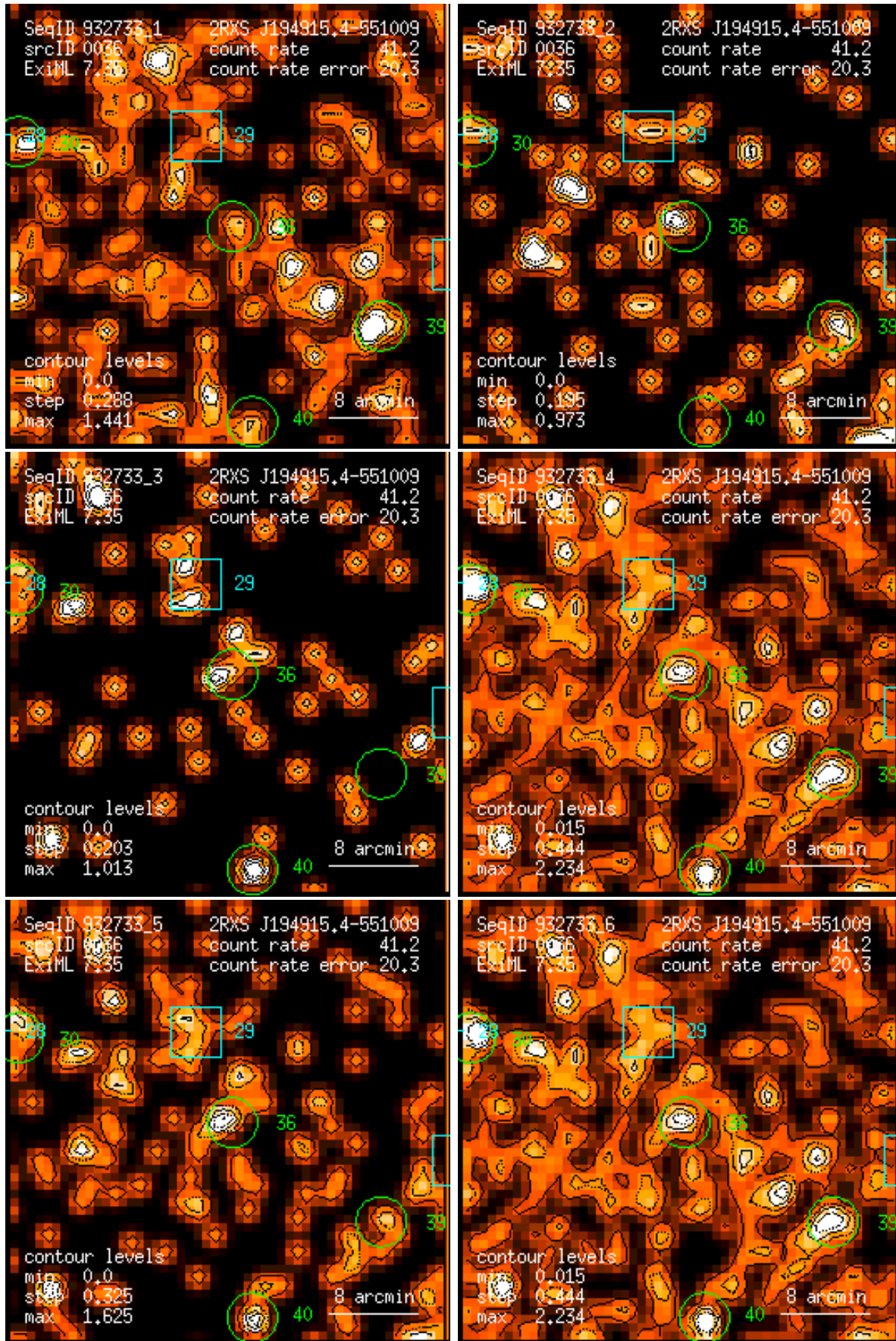
Figure 36: RASS 932733: detection 0036: band rate images, Gaussian filter: (1) PSPC channels 11 – 41, (2) 52 – 90, (3) 91 – 201, (4) 11 – 235, (5) 52 – 201, (6) 11 – 201. Broad band rates in counts/ks. Band rate contour levels in counts/ks/arcmin 2 .
