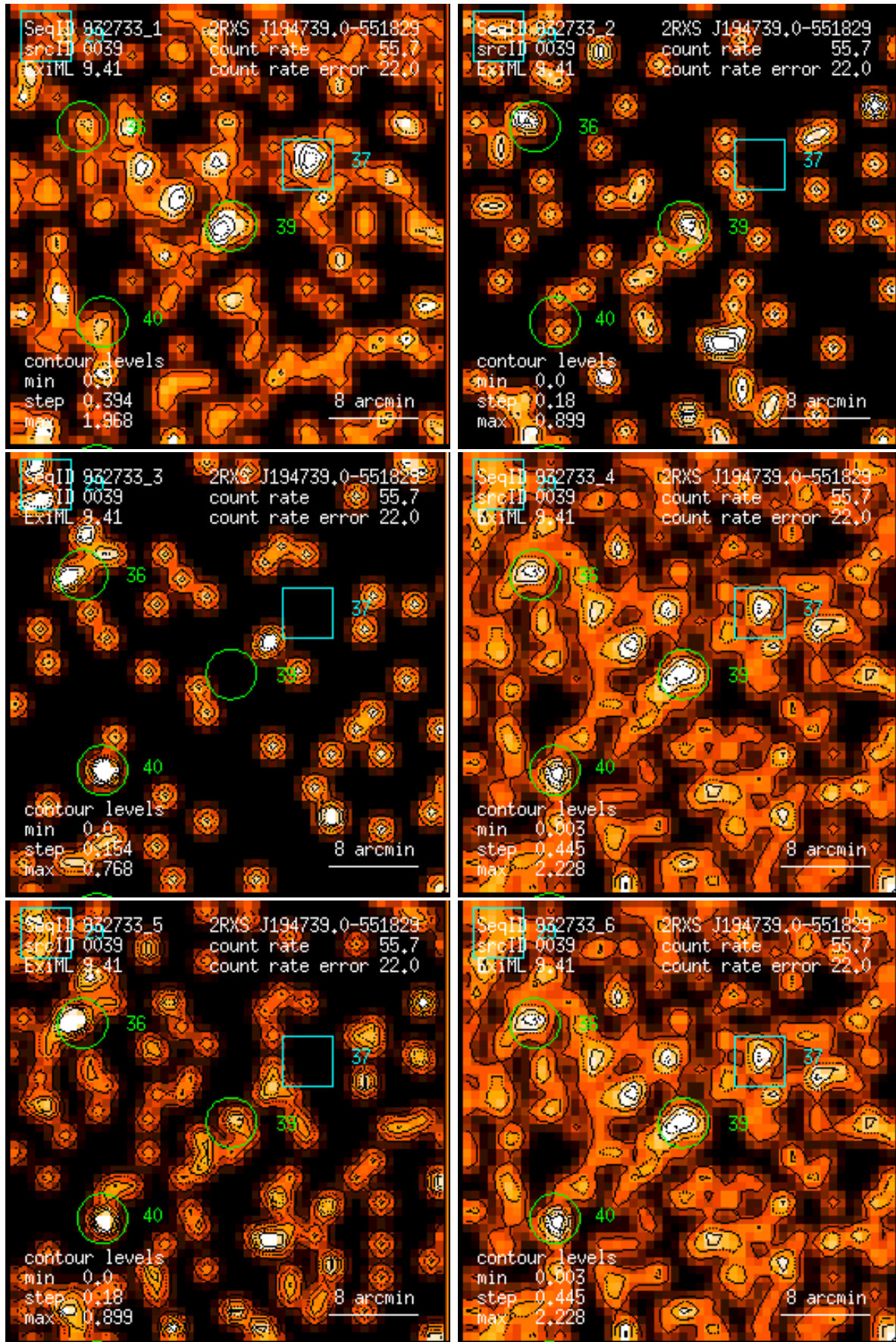
Figure 39: RASS 932733: detection 0039: band rate images, Gaussian filter: (1) PSPC channels 11 – 41, (2) 52 – 90, (3) 91 – 201, (4) 11 – 235, (5) 52 – 201, (6) 11 – 201. Broad band rates in counts/ks. Band rate contour levels in counts/ks/arcmin 2 .
