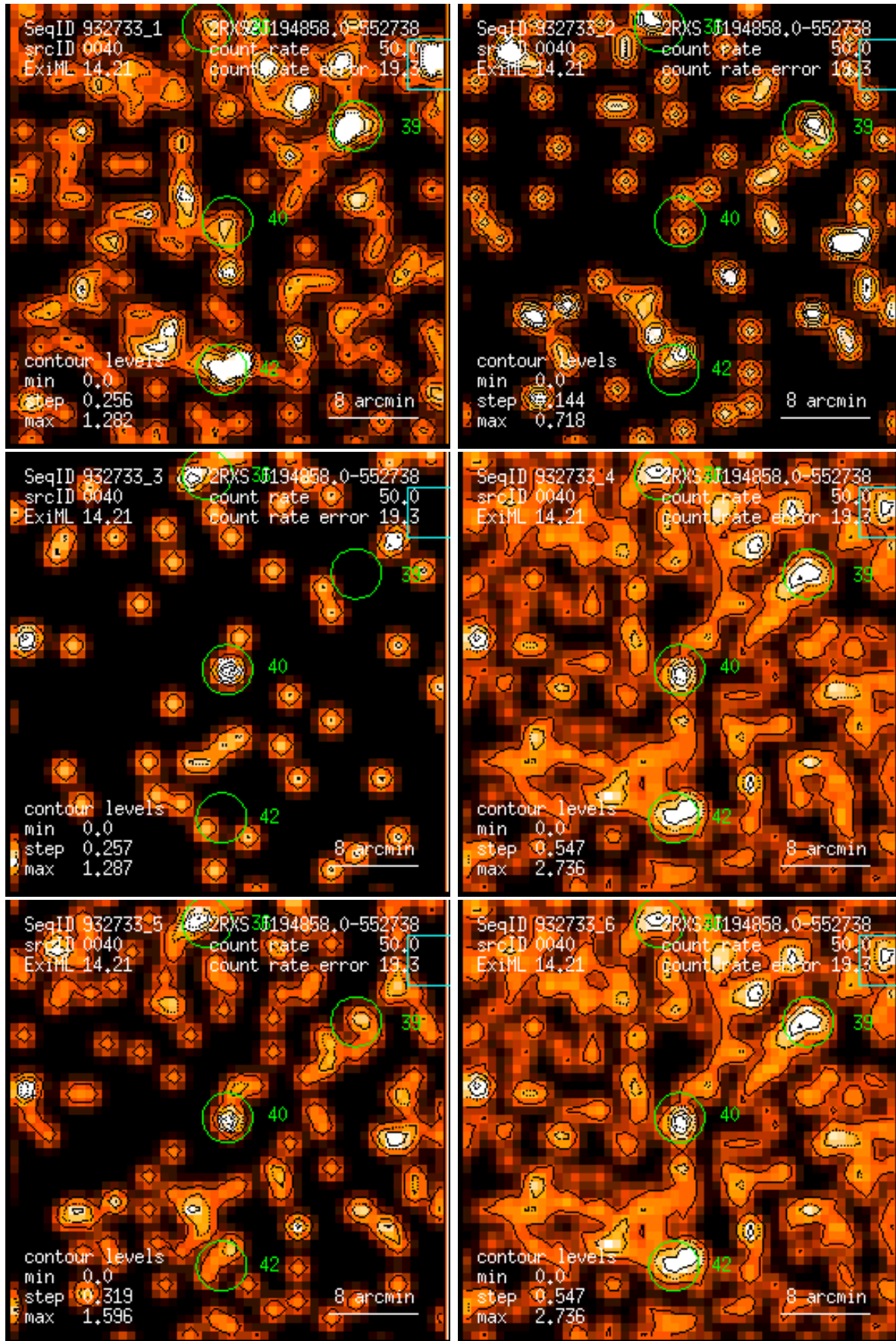
Figure 40: RASS 932733: detection 0040: band rate images, Gaussian filter: (1) PSPC channels 11 – 41, (2) 52 – 90, (3) 91 – 201, (4) 11 – 235, (5) 52 – 201, (6) 11 – 201. Broad band rates in counts/ks. Band rate contour levels in counts/ks/arcmin 2 .
