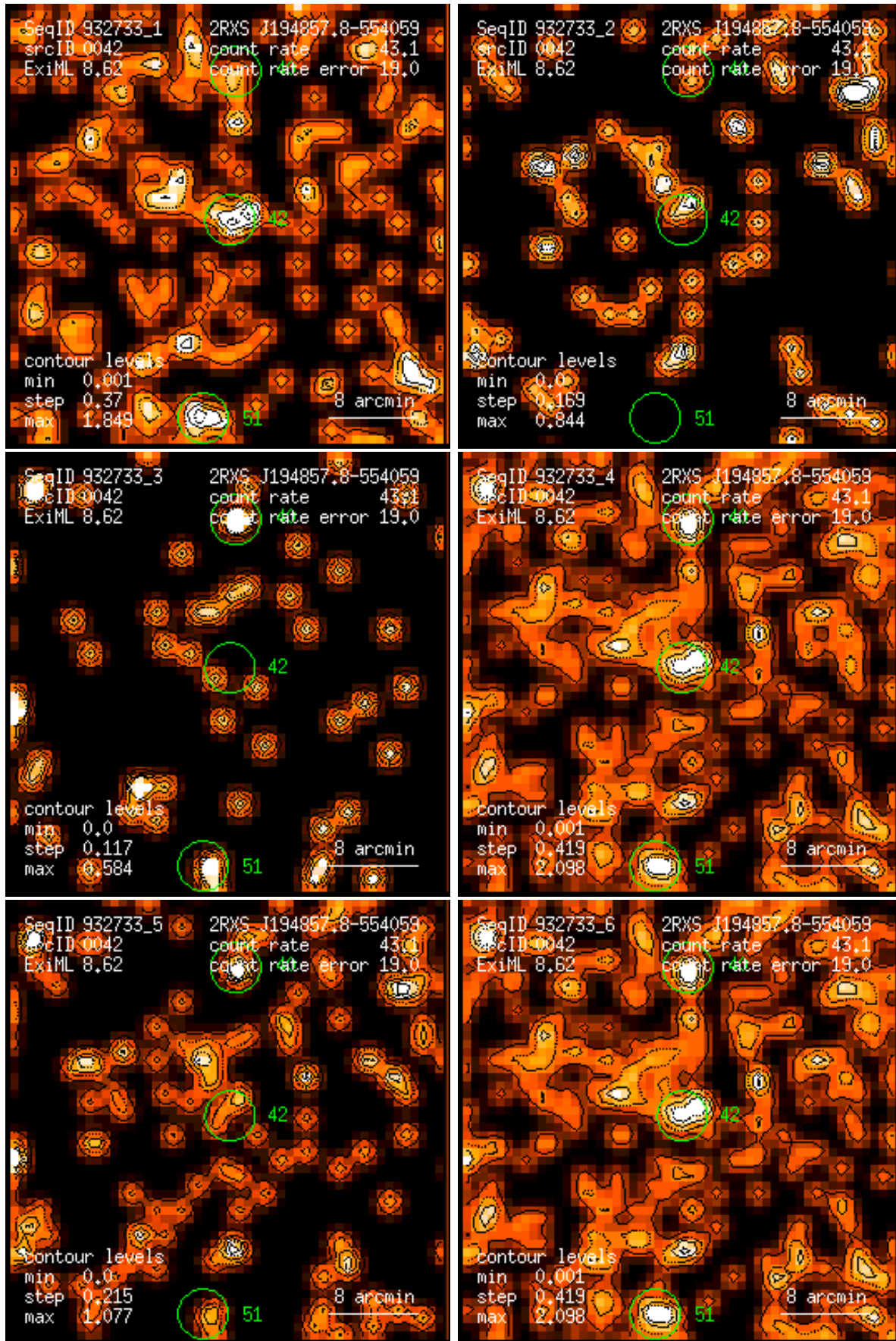
Figure 42: RASS 932733: detection 0042: band rate images, Gaussian filter: (1) PSPC channels 11 – 41, (2) 52 – 90, (3) 91 – 201, (4) 11 – 235, (5) 52 – 201, (6) 11 – 201. Broad band rates in counts/ks. Band rate contour levels in counts/ks/arcmin 2 .
