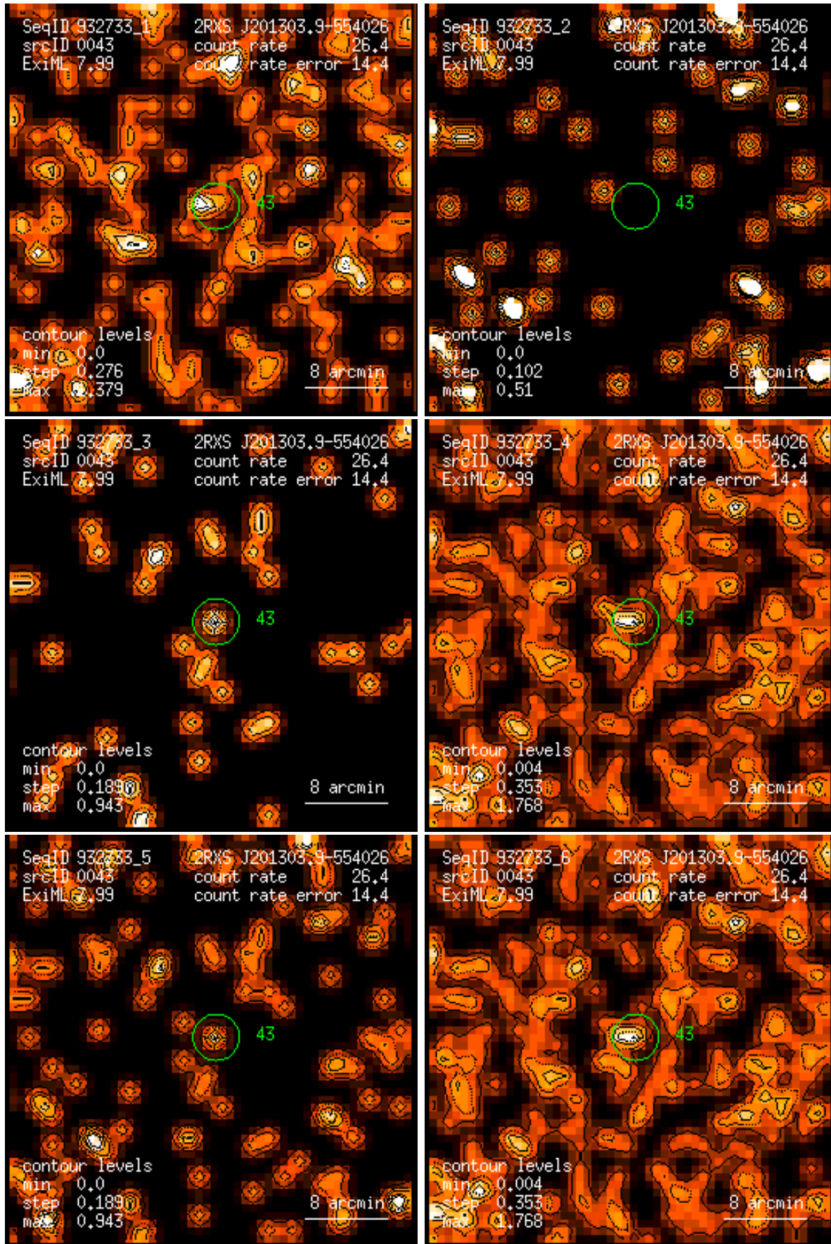
Figure 43: RASS 932733: detection 0043: band rate images, Gaussian filter: (1) PSPC channels 11 – 41, (2) 52 – 90, (3) 91 – 201, (4) 11 – 235, (5) 52 – 201, (6) 11 – 201. Broad band rates in counts/ks. Band rate contour levels in counts/ks/arcmin 2 .
