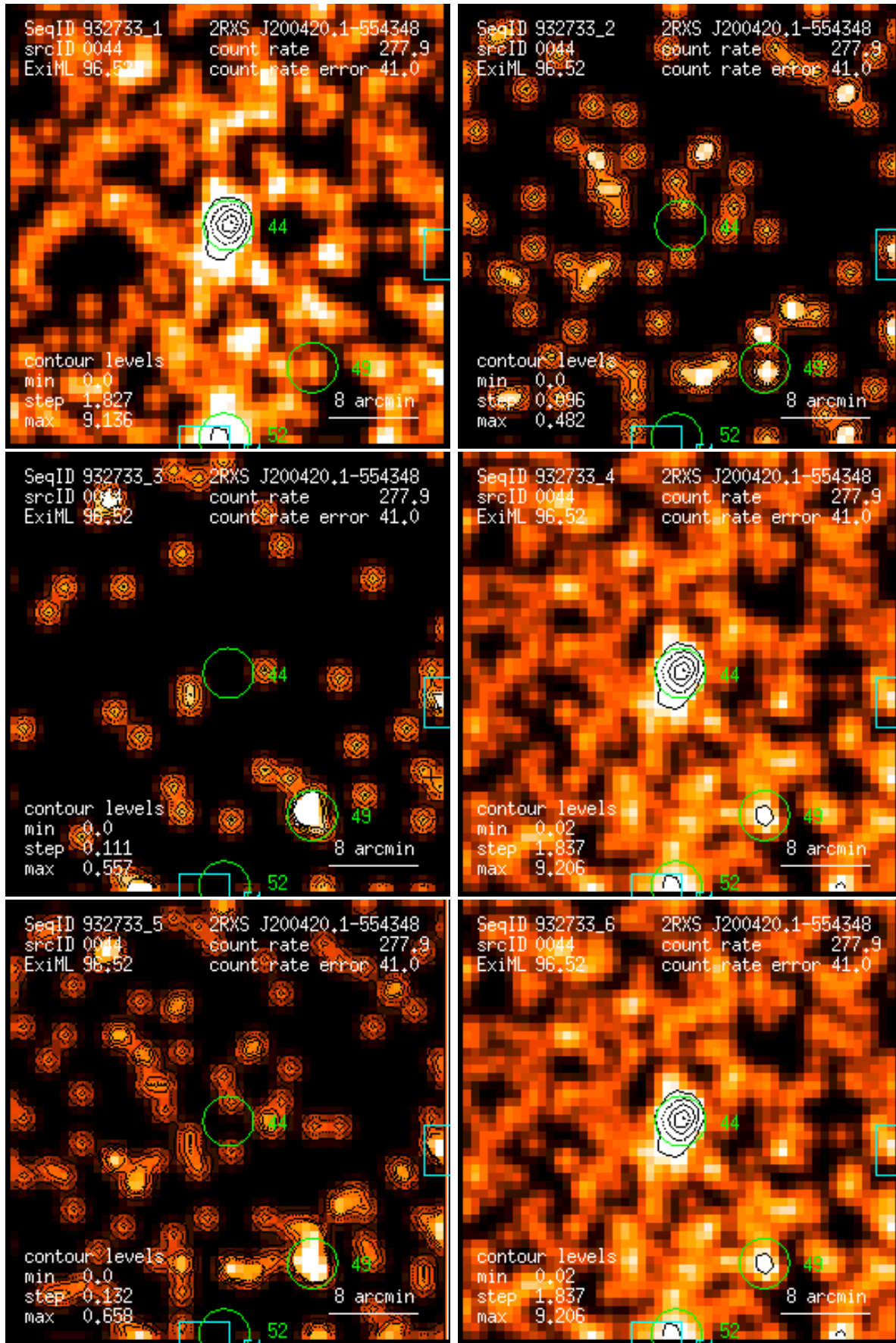
Figure 44: RASS 932733: detection 0044: band rate images, Gaussian filter: (1) PSPC channels 11 – 41, (2) 52 – 90, (3) 91 – 201, (4) 11 – 235, (5) 52 – 201, (6) 11 – 201. Broad band rates in counts/ks. Band rate contour levels in counts/ks/arcmin 2 .
